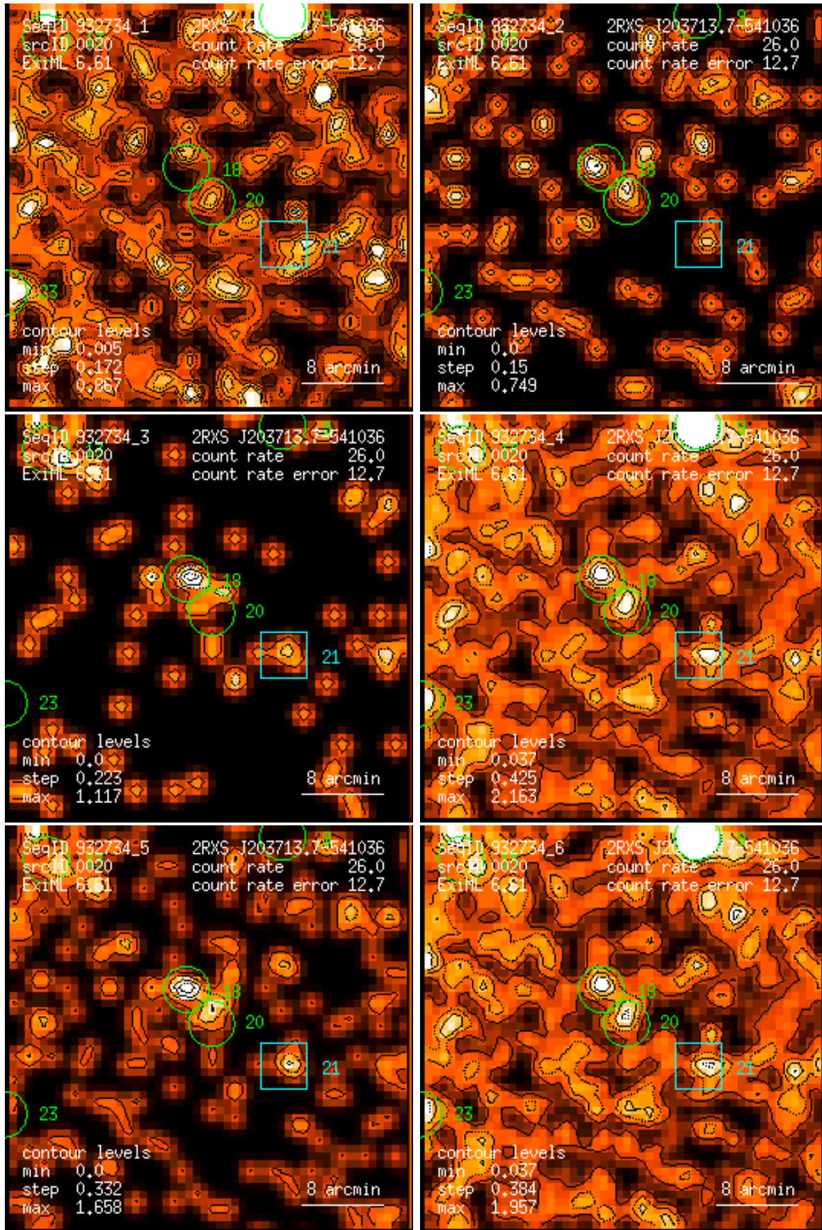
Figure 20: RASS 932734: detection 0020: band rate images, Gaussian filter: (1) PSPC channels 11 – 41, (2) 52 – 90, (3) 91 – 201, (4) 11 – 235, (5) 52 – 201, (6) 11 – 201. Broad band rates in counts/ks. Band rate contour levels in counts/ks/arcmin 2 .
