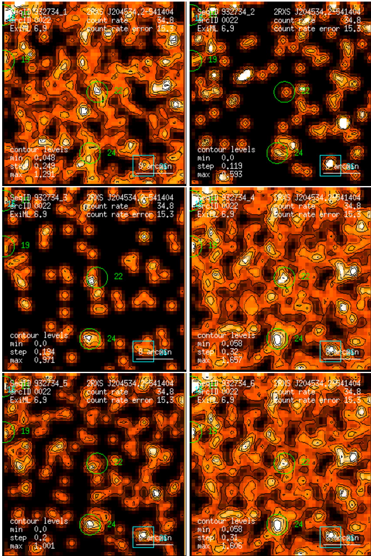
Figure 22: RASS 932734: detection 0022: band rate images, Gaussian filter: (1) PSPC channels 11 – 41, (2) 52 – 90, (3) 91 – 201, (4) 11 – 235, (5) 52 – 201, (6) 11 – 201. Broad band rates in counts/ks. Band rate contour levels in counts/ks/arcmin 2 .
