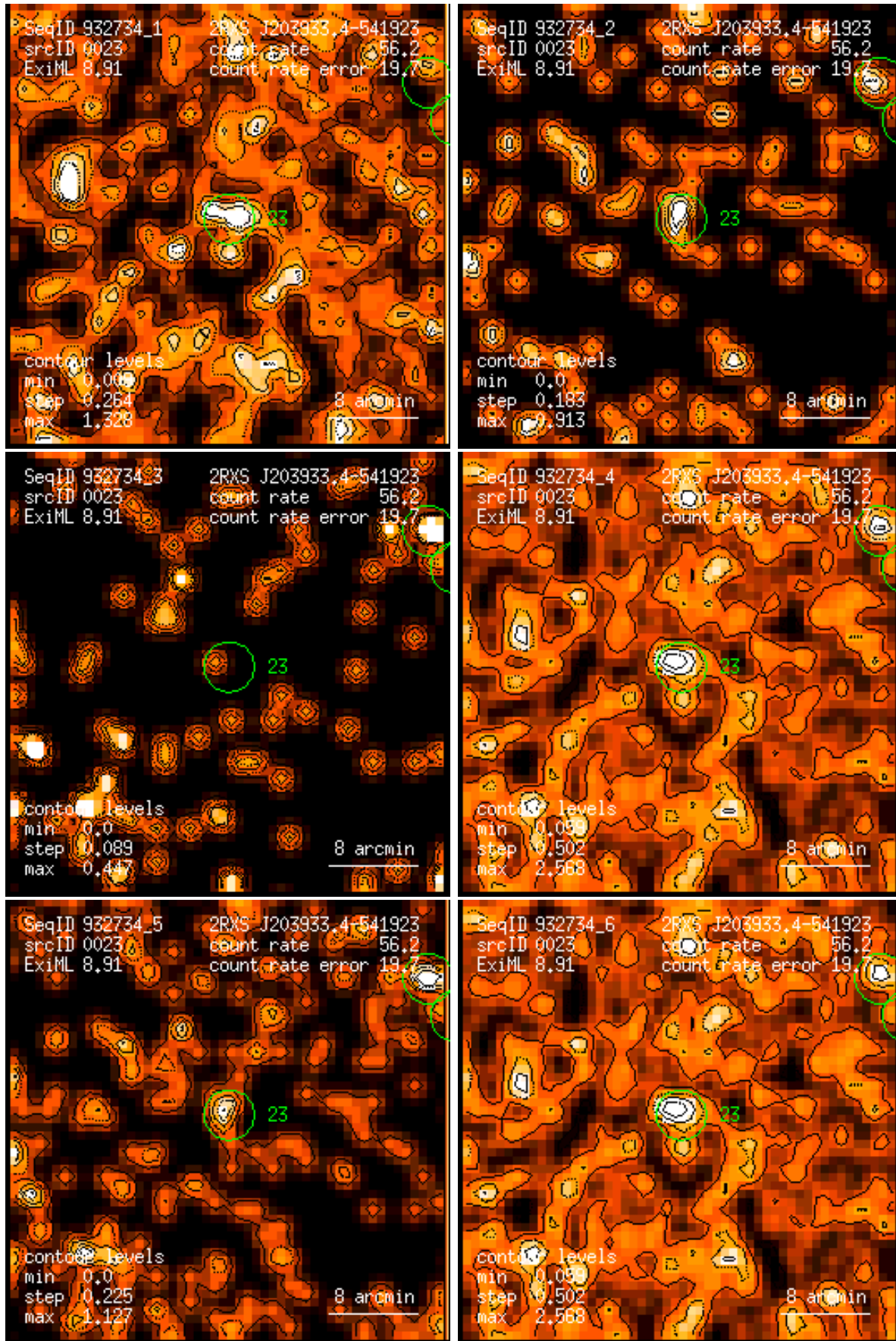
Figure 23: RASS 932734: detection 0023: band rate images, Gaussian filter: (1) PSPC channels 11 – 41, (2) 52 – 90, (3) 91 – 201, (4) 11 – 235, (5) 52 – 201, (6) 11 – 201. Broad band rates in counts/ks. Band rate contour levels in counts/ks/arcmin 2 .
