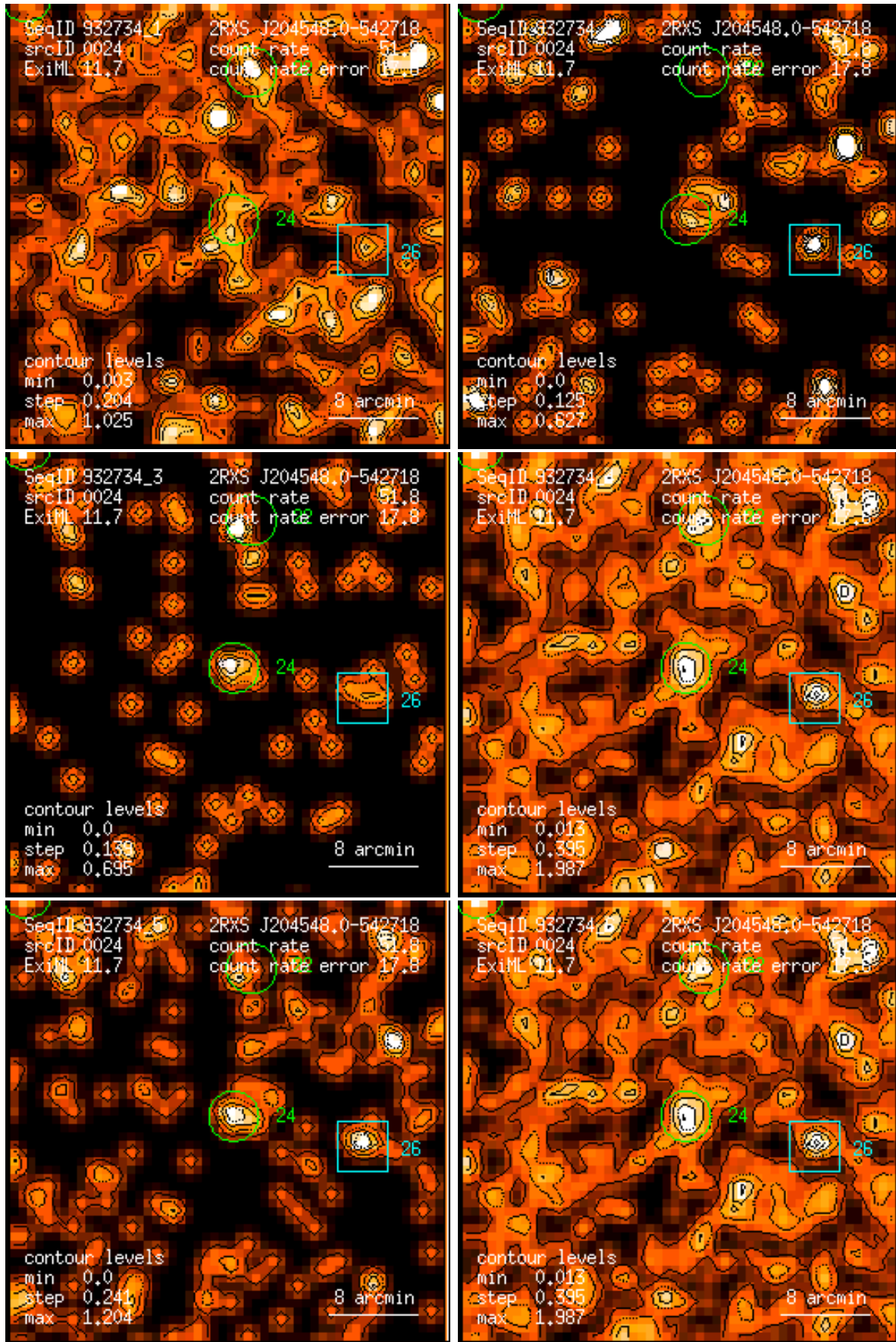
Figure 24: RASS 932734: detection 0024: band rate images, Gaussian filter: (1) PSPC channels 11 – 41, (2) 52 – 90, (3) 91 – 201, (4) 11 – 235, (5) 52 – 201, (6) 11 – 201. Broad band rates in counts/ks. Band rate contour levels in counts/ks/arcmin 2 .
