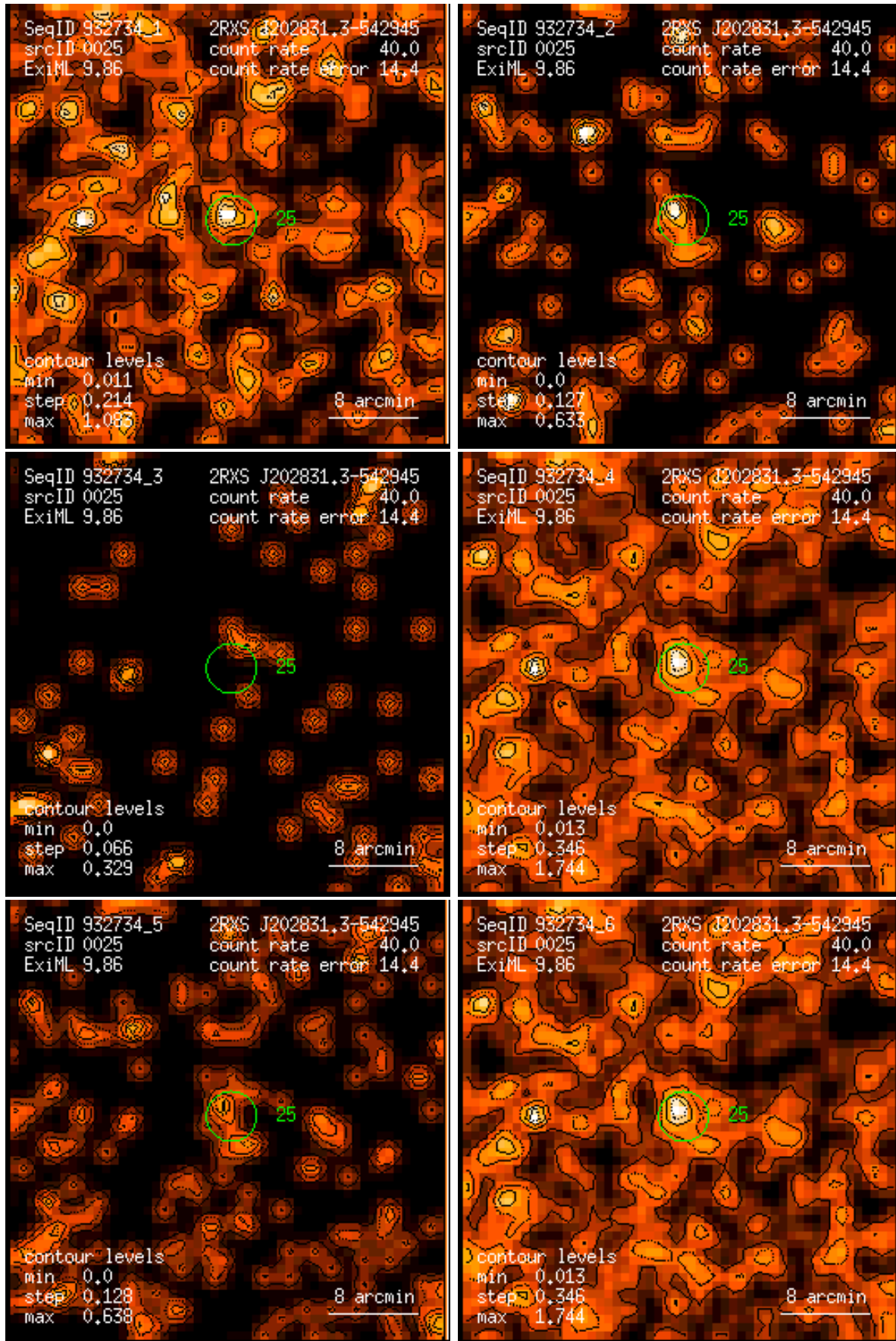
Figure 25: RASS 932734: detection 0025: band rate images, Gaussian filter: (1) PSPC channels 11 – 41, (2) 52 – 90, (3) 91 – 201, (4) 11 – 235, (5) 52 – 201, (6) 11 – 201. Broad band rates in counts/ks. Band rate contour levels in counts/ks/arcmin 2 .
