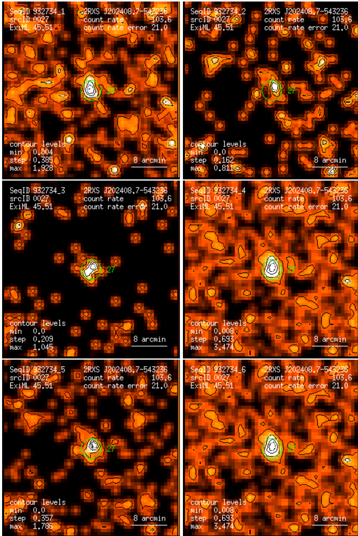
Figure 27: RASS 932734: detection 0027: band rate images, Gaussian filter: (1) PSPC channels 11 – 41, (2) 52 – 90, (3) 91 – 201, (4) 11 – 235, (5) 52 – 201, (6) 11 – 201. Broad band rates in counts/ks. Band rate contour levels in counts/ks/arcmin 2 .
