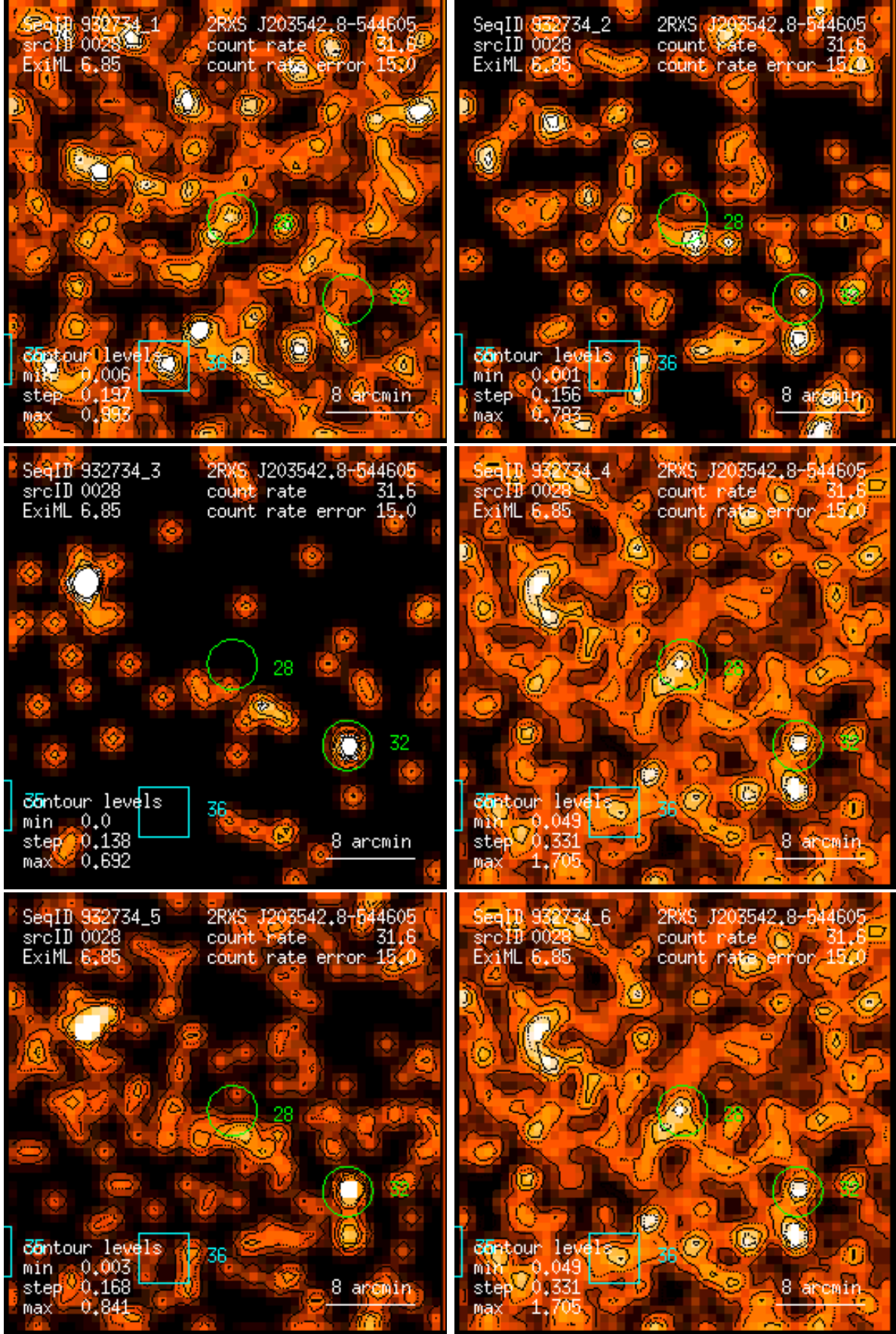
Figure 28: RASS 932734: detection 0028: band rate images, Gaussian filter: (1) PSPC channels 11 – 41, (2) 52 – 90, (3) 91 – 201, (4) 11 – 235, (5) 52 – 201, (6) 11 – 201. Broad band rates in counts/ks. Band rate contour levels in counts/ks/arcmin 2 .
