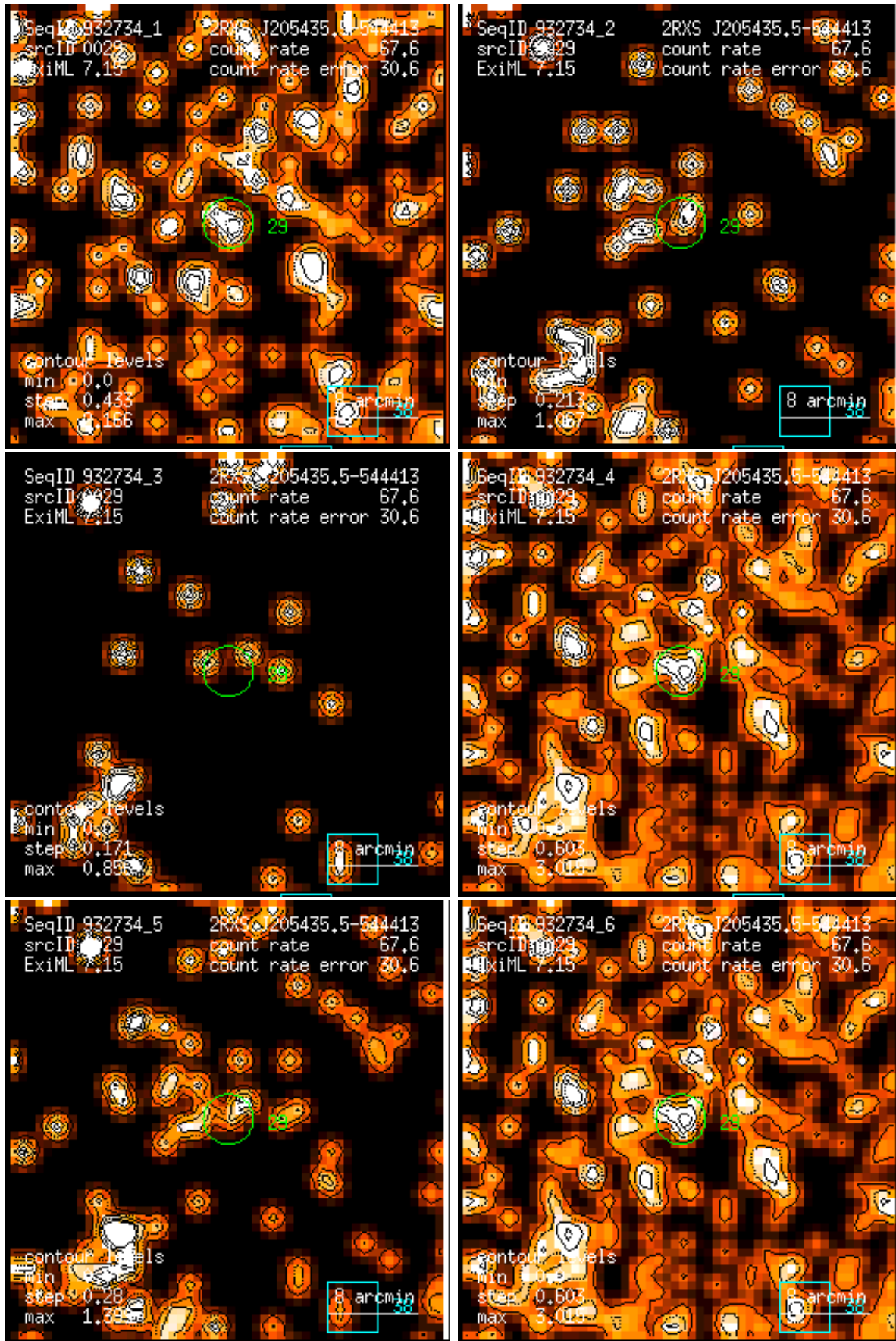
Figure 29: RASS 932734: detection 0029: band rate images, Gaussian filter: (1) PSPC channels 11 – 41, (2) 52 – 90, (3) 91 – 201, (4) 11 – 235, (5) 52 – 201, (6) 11 – 201. Broad band rates in counts/ks. Band rate contour levels in counts/ks/arcmin 2 .
