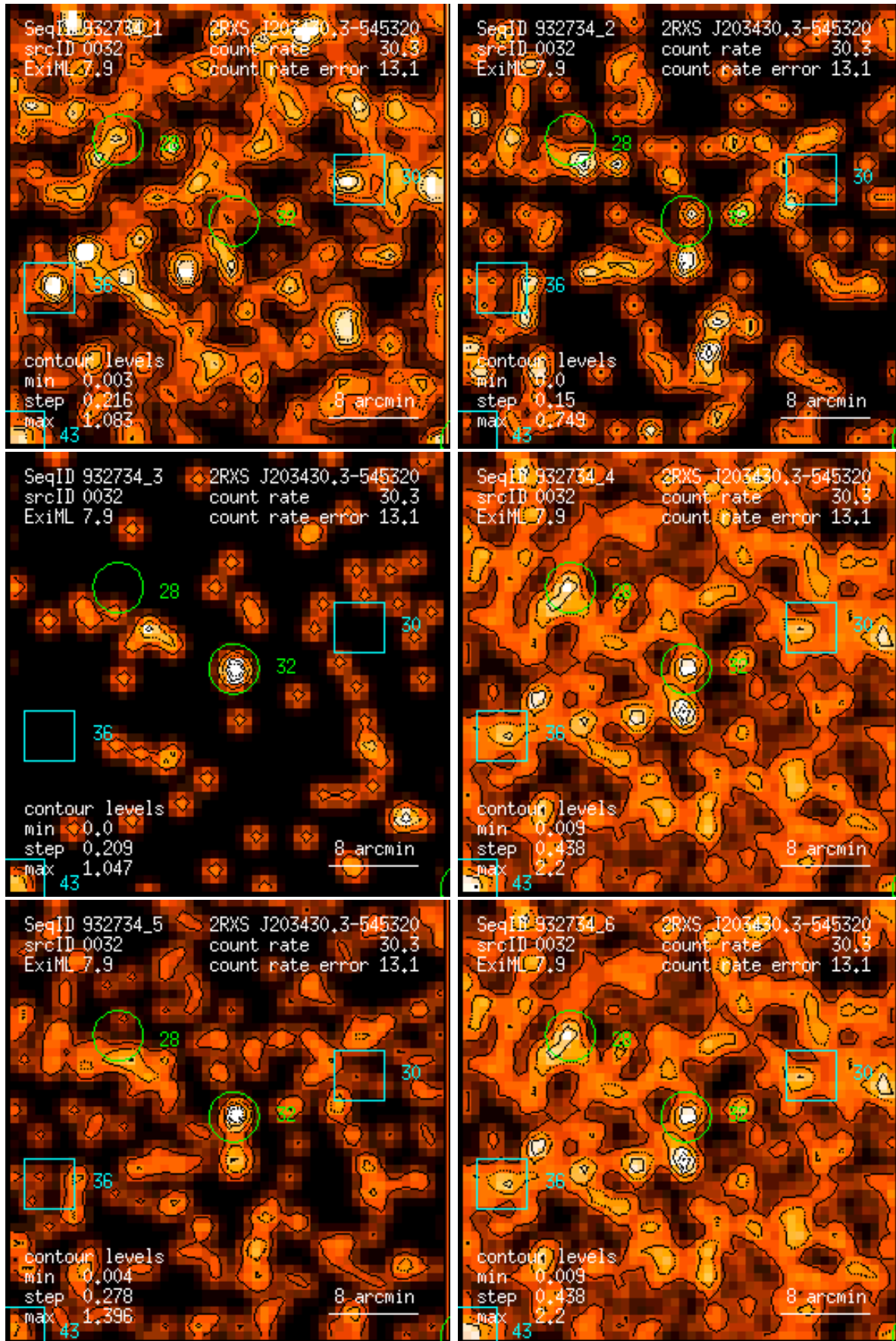
Figure 32: RASS 932734: detection 0032: band rate images, Gaussian filter: (1) PSPC channels 11 – 41, (2) 52 – 90, (3) 91 – 201, (4) 11 – 235, (5) 52 – 201, (6) 11 – 201. Broad band rates in counts/ks. Band rate contour levels in counts/ks/arcmin 2 .
