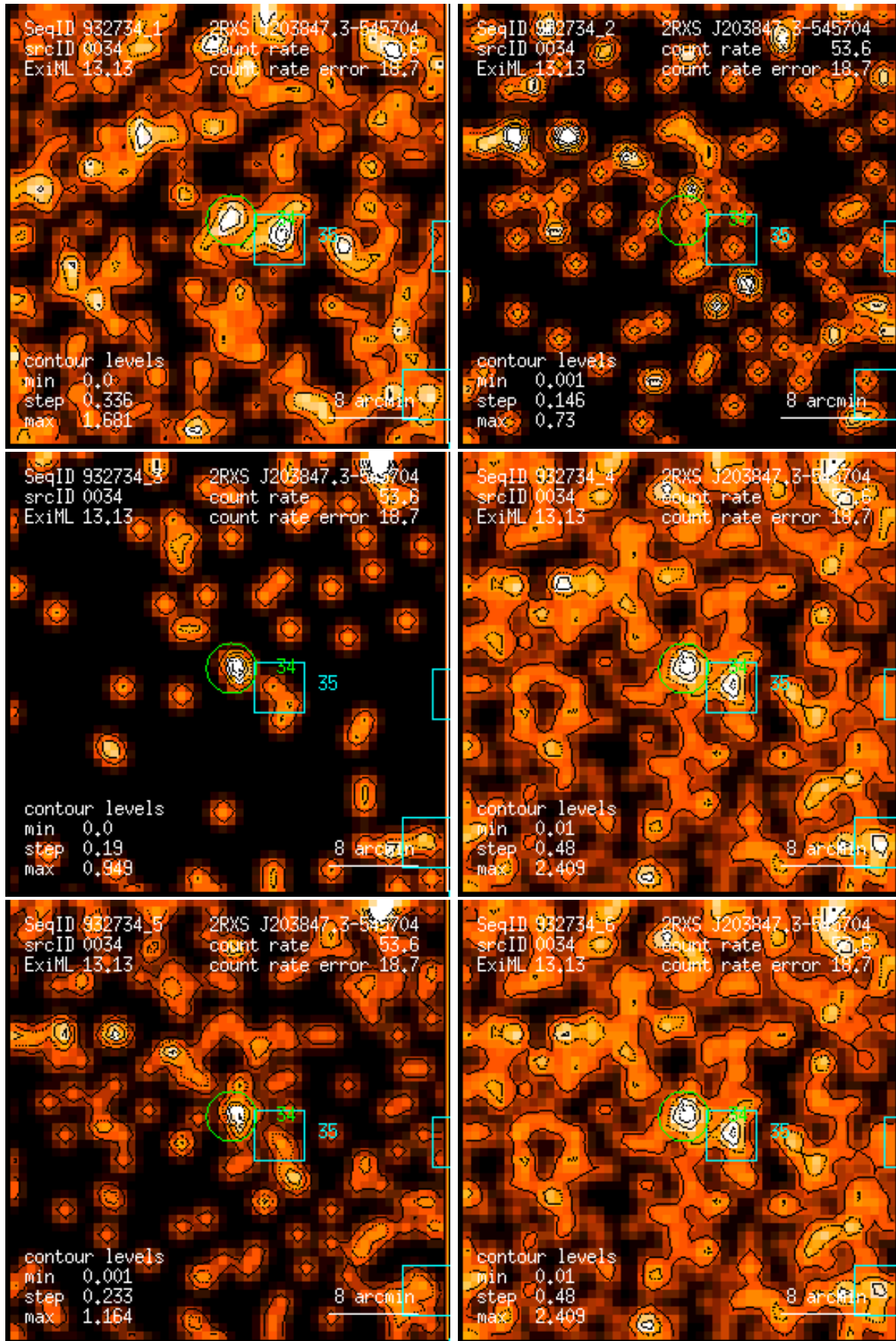
Figure 34: RASS 932734: detection 0034: band rate images, Gaussian filter: (1) PSPC channels 11 – 41, (2) 52 – 90, (3) 91 – 201, (4) 11 – 235, (5) 52 – 201, (6) 11 – 201. Broad band rates in counts/ks. Band rate contour levels in counts/ks/arcmin 2 .
