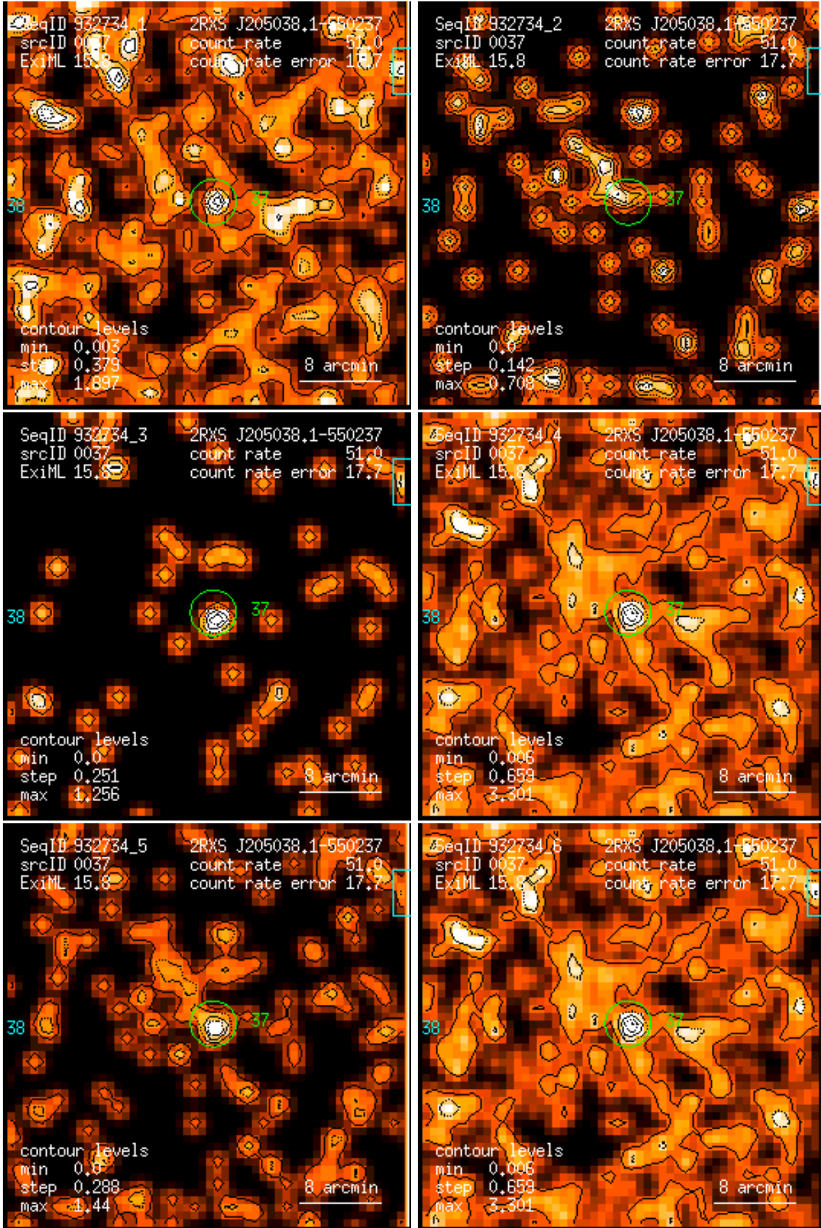
Figure 37: RASS 932734: detection 0037: band rate images, Gaussian filter: (1) PSPC channels 11 – 41, (2) 52 – 90, (3) 91 – 201, (4) 11 – 235, (5) 52 – 201, (6) 11 – 201. Broad band rates in counts/ks. Band rate contour levels in counts/ks/arcmin 2 .
