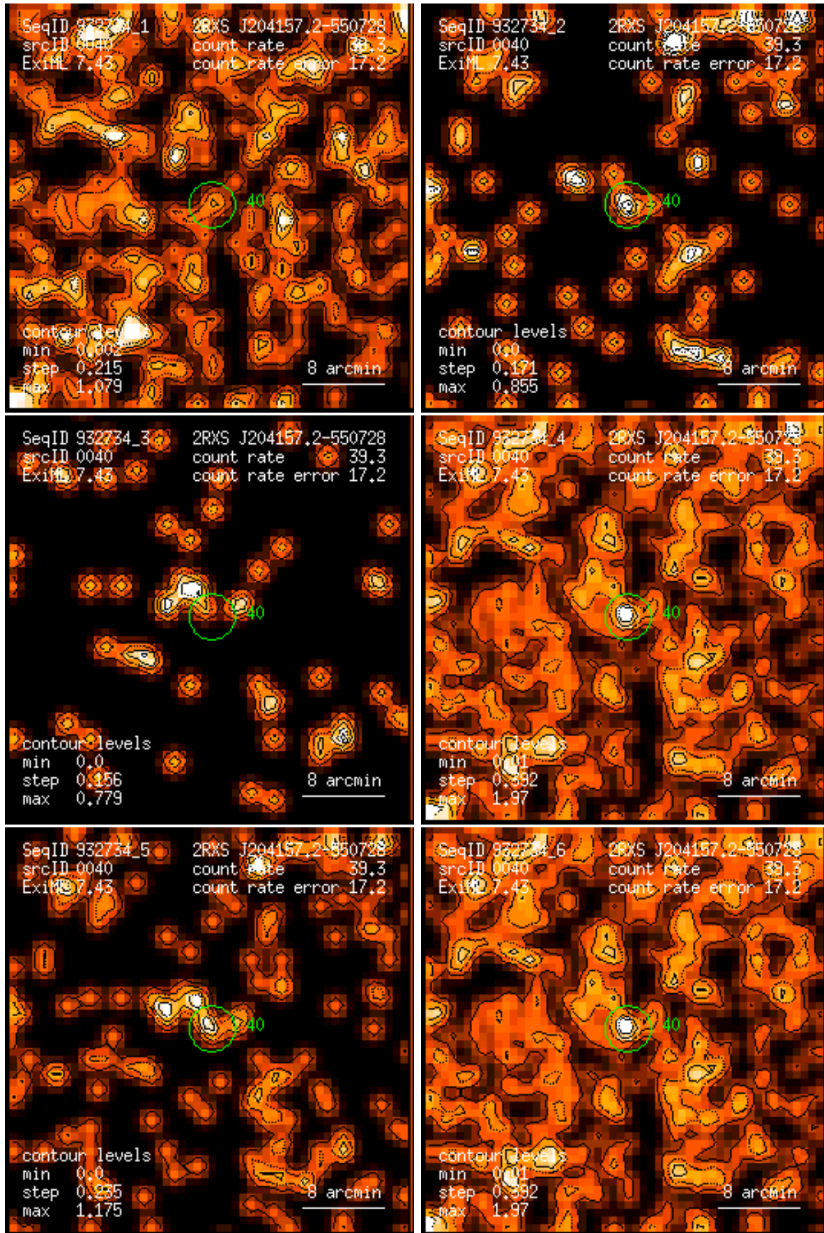
Figure 40: RASS 932734: detection 0040: band rate images, Gaussian filter: (1) PSPC channels 11 – 41, (2) 52 – 90, (3) 91 – 201, (4) 11 – 235, (5) 52 – 201, (6) 11 – 201. Broad band rates in counts/ks. Band rate contour levels in counts/ks/arcmin 2 .
