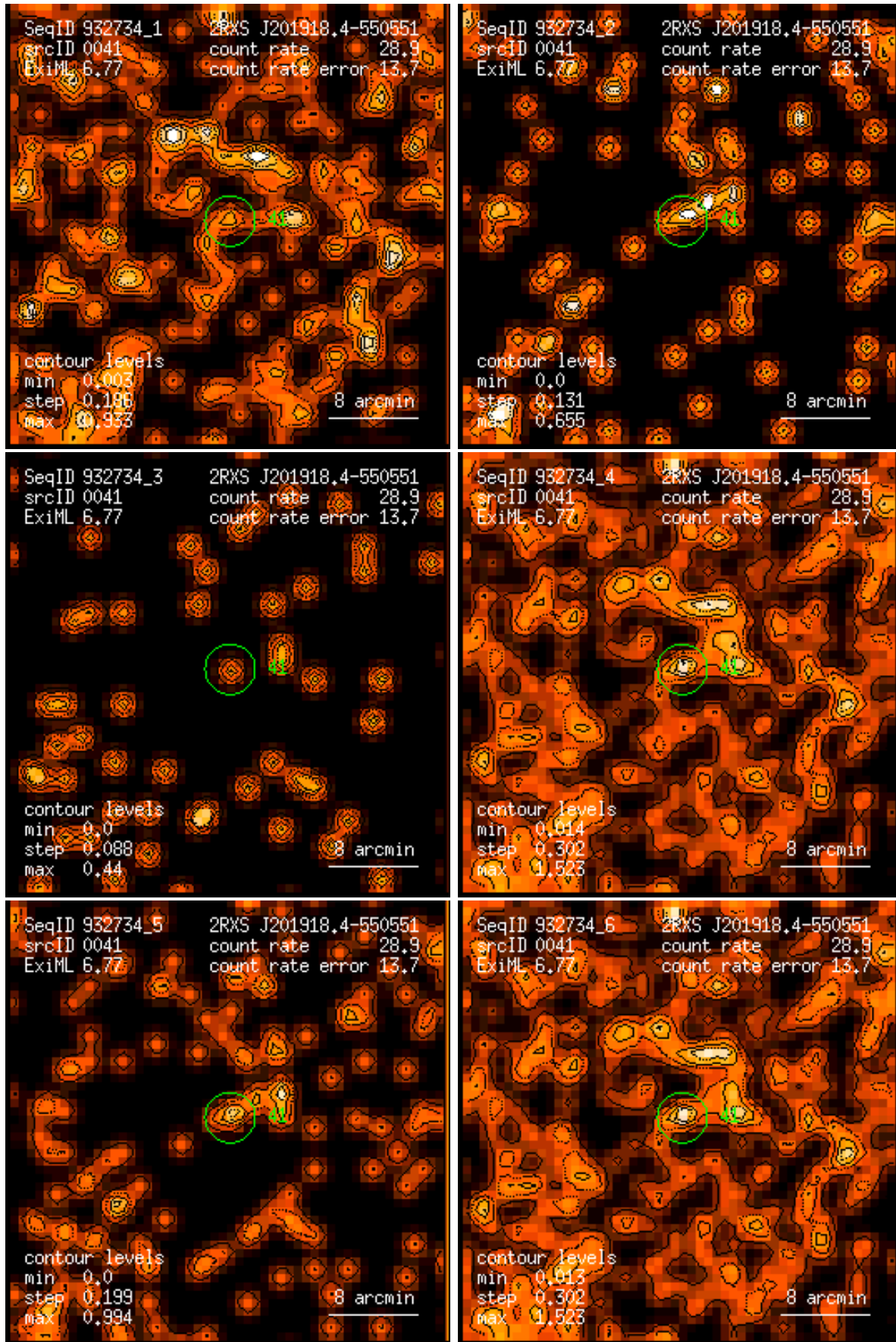
Figure 41: RASS 932734: detection 0041: band rate images, Gaussian filter: (1) PSPC channels 11 – 41, (2) 52 – 90, (3) 91 – 201, (4) 11 – 235, (5) 52 – 201, (6) 11 – 201. Broad band rates in counts/ks. Band rate contour levels in counts/ks/arcmin 2 .
