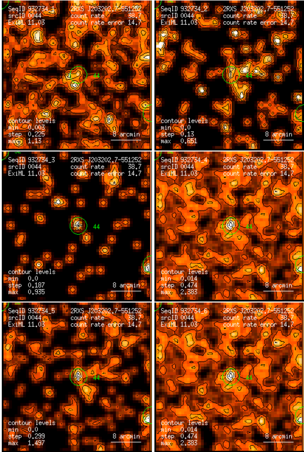
Figure 44: RASS 932734: detection 0044: band rate images, Gaussian filter: (1) PSPC channels 11 – 41, (2) 52 – 90, (3) 91 – 201, (4) 11 – 235, (5) 52 – 201, (6) 11 – 201. Broad band rates in counts/ks. Band rate contour levels in counts/ks/arcmin 2 .
