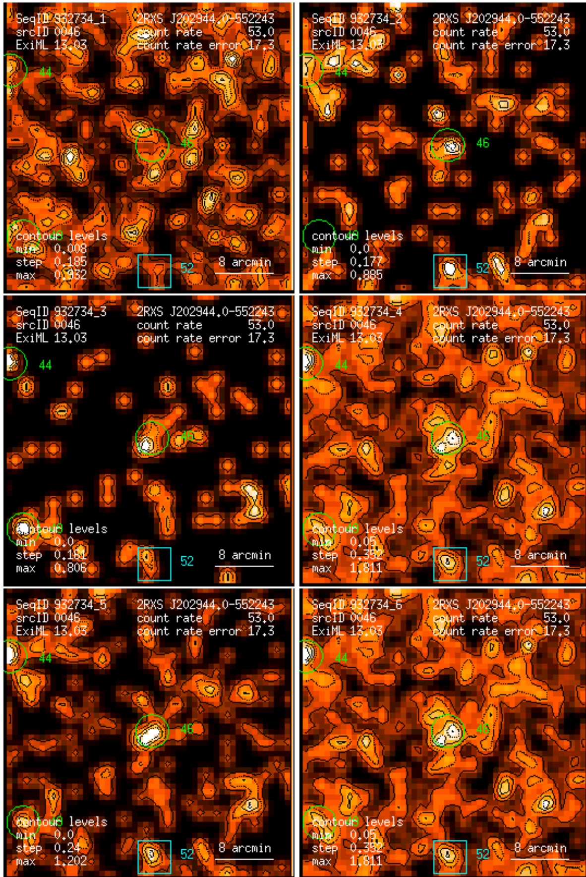
Figure 46: RASS 932734: detection 0046: band rate images, Gaussian filter: (1) PSPC channels 11 – 41, (2) 52 – 90, (3) 91 – 201, (4) 11 – 235, (5) 52 – 201, (6) 11 – 201. Broad band rates in counts/ks. Band rate contour levels in counts/ks/arcmin 2 .
