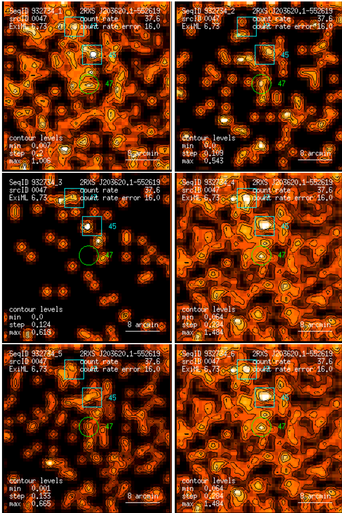
Figure 47: RASS 932734: detection 0047: band rate images, Gaussian filter: (1) PSPC channels 11 – 41, (2) 52 – 90, (3) 91 – 201, (4) 11 – 235, (5) 52 – 201, (6) 11 – 201. Broad band rates in counts/ks. Band rate contour levels in counts/ks/arcmin 2 .
