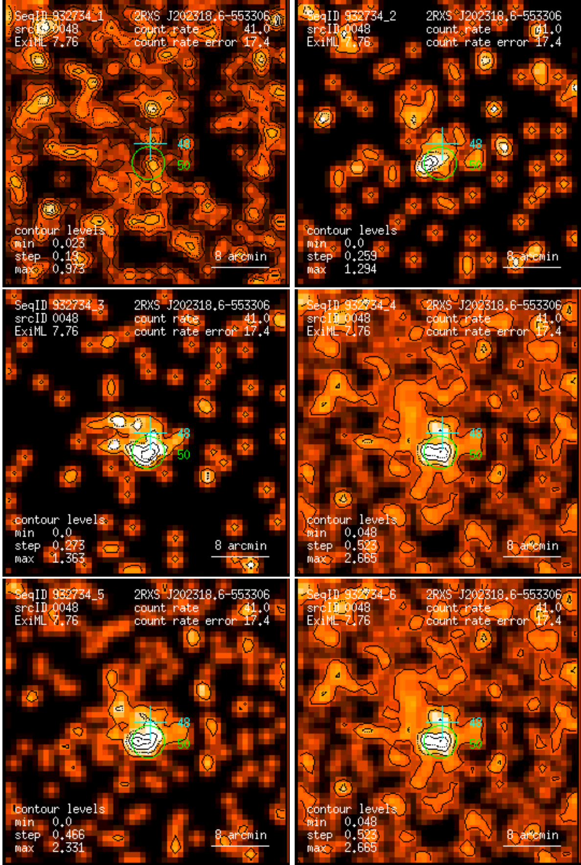
Figure 48: RASS 932734: detection 0048: band rate images, Gaussian filter: (1) PSPC channels 11 – 41, (2) 52 – 90, (3) 91 – 201, (4) 11 – 235, (5) 52 – 201, (6) 11 – 201. Broad band rates in counts/ks. Band rate contour levels in counts/ks/arcmin 2 .
