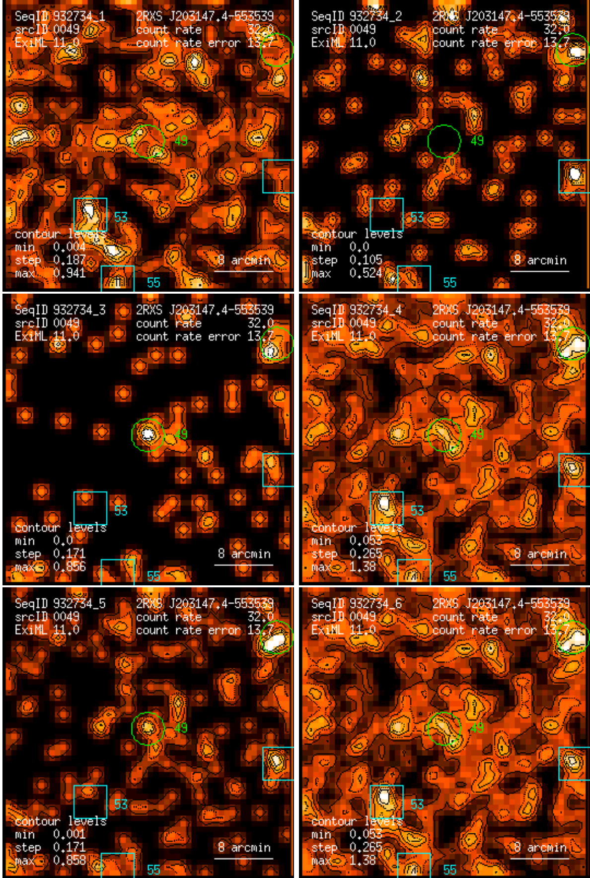
Figure 49: RASS 932734: detection 0049: band rate images, Gaussian filter: (1) PSPC channels 11 – 41, (2) 52 – 90, (3) 91 – 201, (4) 11 – 235, (5) 52 – 201, (6) 11 – 201. Broad band rates in counts/ks. Band rate contour levels in counts/ks/arcmin 2 .
