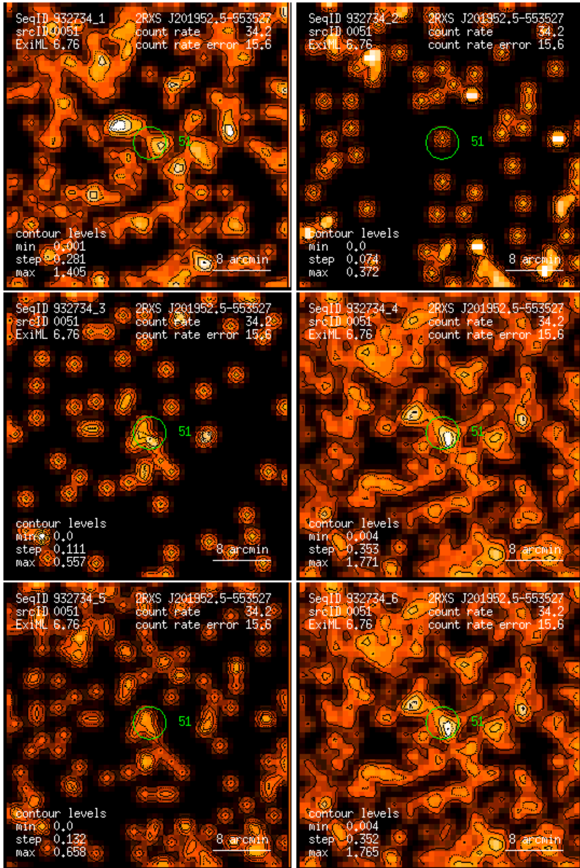
Figure 51: RASS 932734: detection 0051: band rate images, Gaussian filter: (1) PSPC channels 11 – 41, (2) 52 – 90, (3) 91 – 201, (4) 11 – 235, (5) 52 – 201, (6) 11 – 201. Broad band rates in counts/ks. Band rate contour levels in counts/ks/arcmin 2 .
