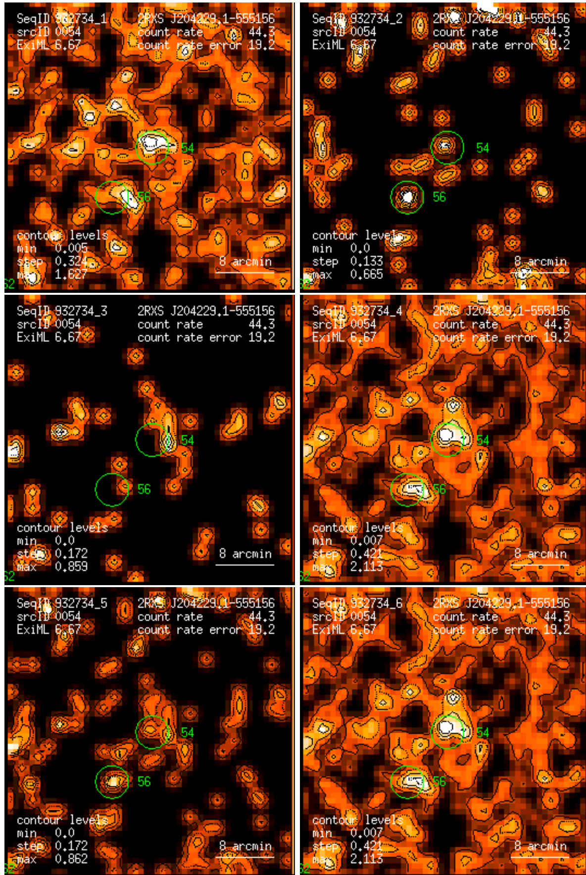
Figure 54: RASS 932734: detection 0054: band rate images, Gaussian filter: (1) PSPC channels 11 – 41, (2) 52 – 90, (3) 91 – 201, (4) 11 – 235, (5) 52 – 201, (6) 11 – 201. Broad band rates in counts/ks. Band rate contour levels in counts/ks/arcmin 2 .
