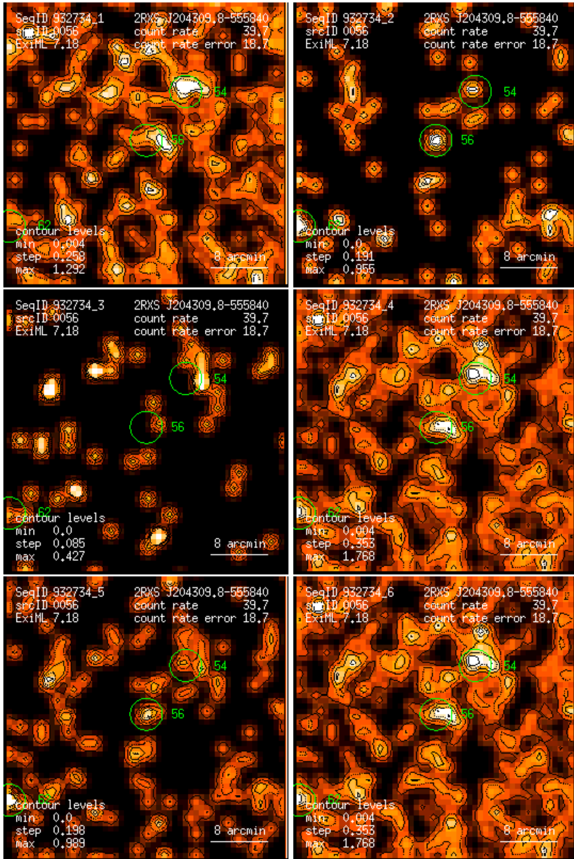
Figure 56: RASS 932734: detection 0056: band rate images, Gaussian filter: (1) PSPC channels 11 – 41, (2) 52 – 90, (3) 91 – 201, (4) 11 – 235, (5) 52 – 201, (6) 11 – 201. Broad band rates in counts/ks. Band rate contour levels in counts/ks/arcmin 2 .
