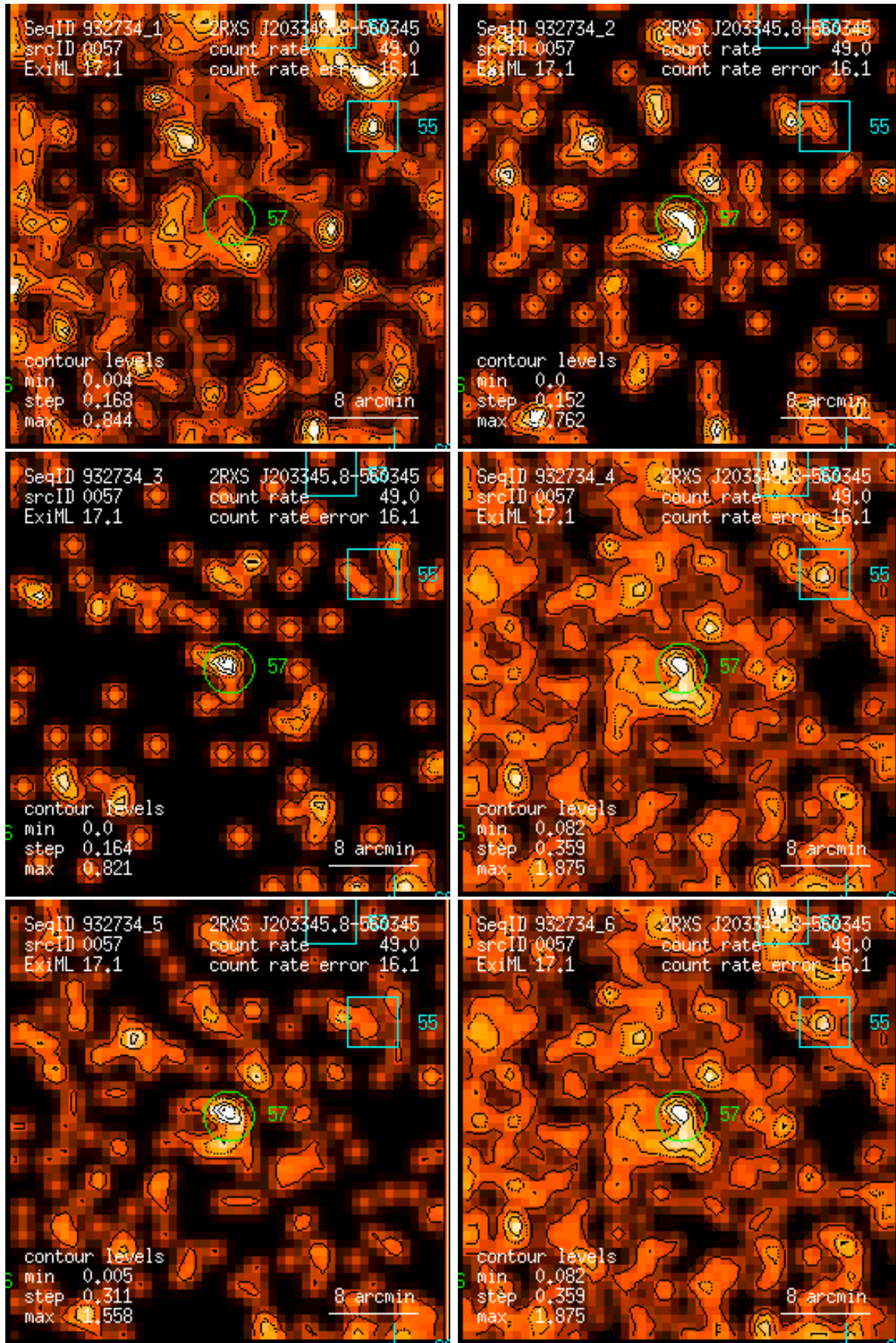
Figure 57: RASS 932734: detection 0057: band rate images, Gaussian filter: (1) PSPC channels 11 – 41, (2) 52 – 90, (3) 91 – 201, (4) 11 – 235, (5) 52 – 201, (6) 11 – 201. Broad band rates in counts/ks. Band rate contour levels in counts/ks/arcmin 2 .
