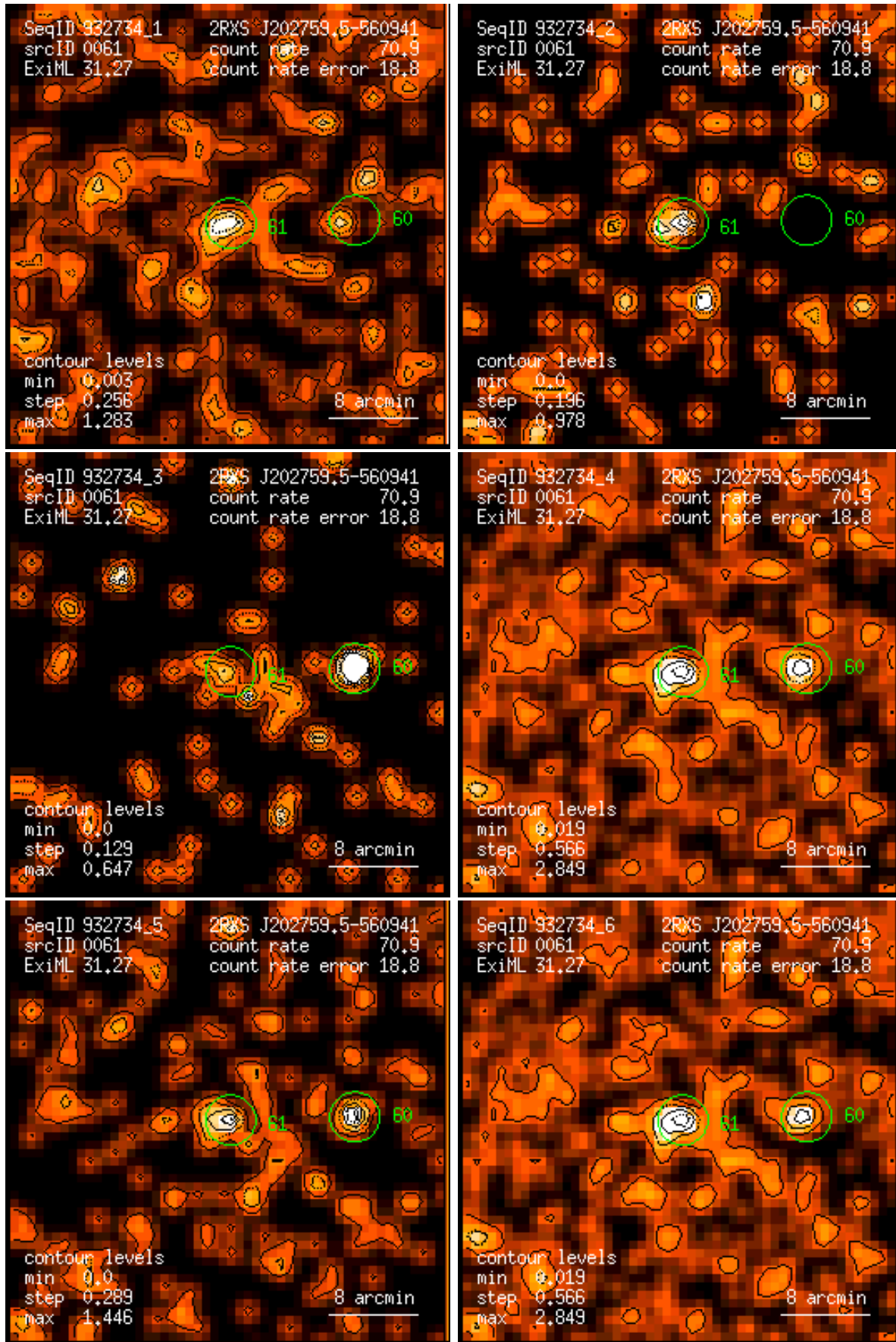
Figure 61: RASS 932734: detection 0061: band rate images, Gaussian filter: (1) PSPC channels 11 – 41, (2) 52 – 90, (3) 91 – 201, (4) 11 – 235, (5) 52 – 201, (6) 11 – 201. Broad band rates in counts/ks. Band rate contour levels in counts/ks/arcmin 2 .
