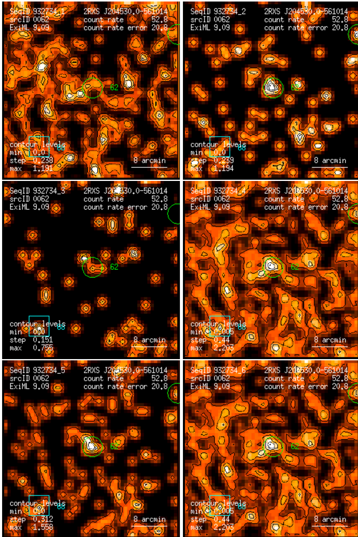
Figure 62: RASS 932734: detection 0062: band rate images, Gaussian filter: (1) PSPC channels 11 – 41, (2) 52 – 90, (3) 91 – 201, (4) 11 – 235, (5) 52 – 201, (6) 11 – 201. Broad band rates in counts/ks. Band rate contour levels in counts/ks/arcmin 2 .
