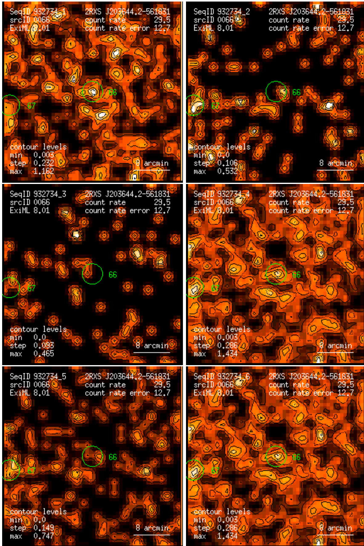
Figure 66: RASS 932734: detection 0066: band rate images, Gaussian filter: (1) PSPC channels 11 – 41, (2) 52 – 90, (3) 91 – 201, (4) 11 – 235, (5) 52 – 201, (6) 11 – 201. Broad band rates in counts/ks. Band rate contour levels in counts/ks/arcmin 2 .
