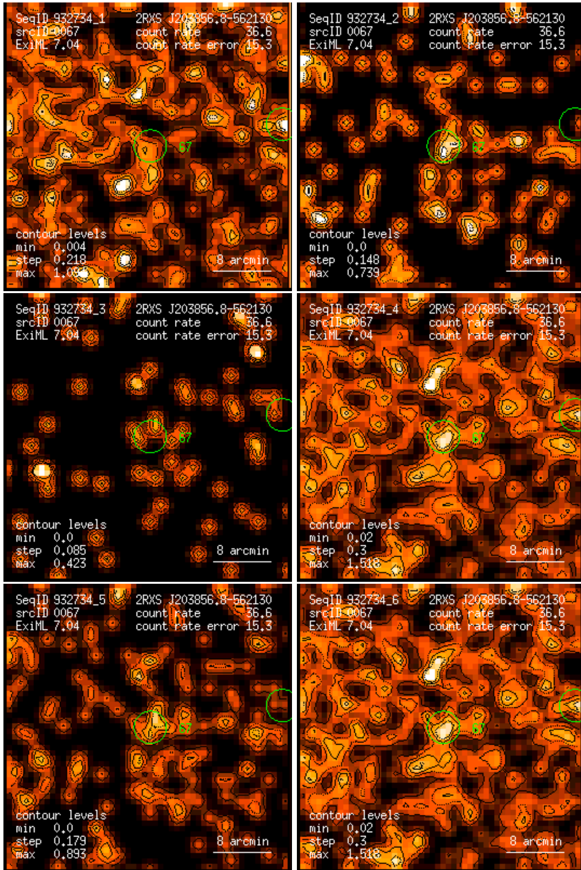
Figure 67: RASS 932734: detection 0067: band rate images, Gaussian filter: (1) PSPC channels 11 – 41, (2) 52 – 90, (3) 91 – 201, (4) 11 – 235, (5) 52 – 201, (6) 11 – 201. Broad band rates in counts/ks. Band rate contour levels in counts/ks/arcmin 2 .
