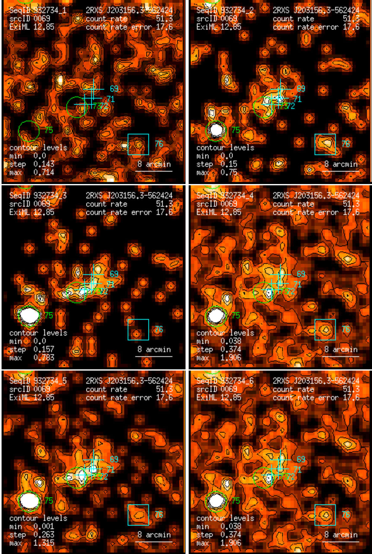
Figure 69: RASS 932734: detection 0069: band rate images, Gaussian filter: (1) PSPC channels 11 – 41, (2) 52 – 90, (3) 91 – 201, (4) 11 – 235, (5) 52 – 201, (6) 11 – 201. Broad band rates in counts/ks. Band rate contour levels in counts/ks/arcmin 2 .
