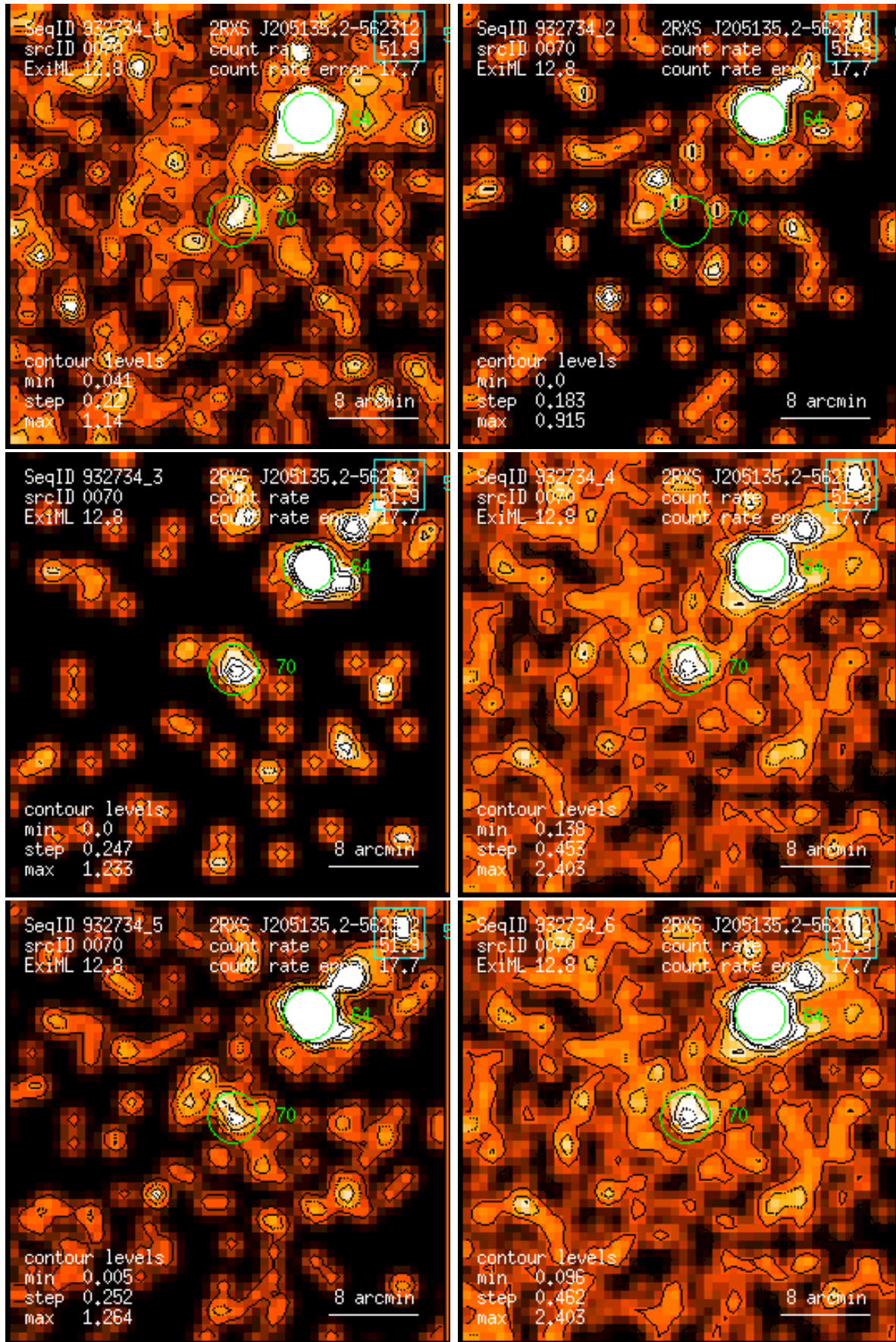
Figure 70: RASS 932734: detection 0070: band rate images, Gaussian filter: (1) PSPC channels 11 – 41, (2) 52 – 90, (3) 91 – 201, (4) 11 – 235, (5) 52 – 201, (6) 11 – 201. Broad band rates in counts/ks. Band rate contour levels in counts/ks/arcmin 2 .
