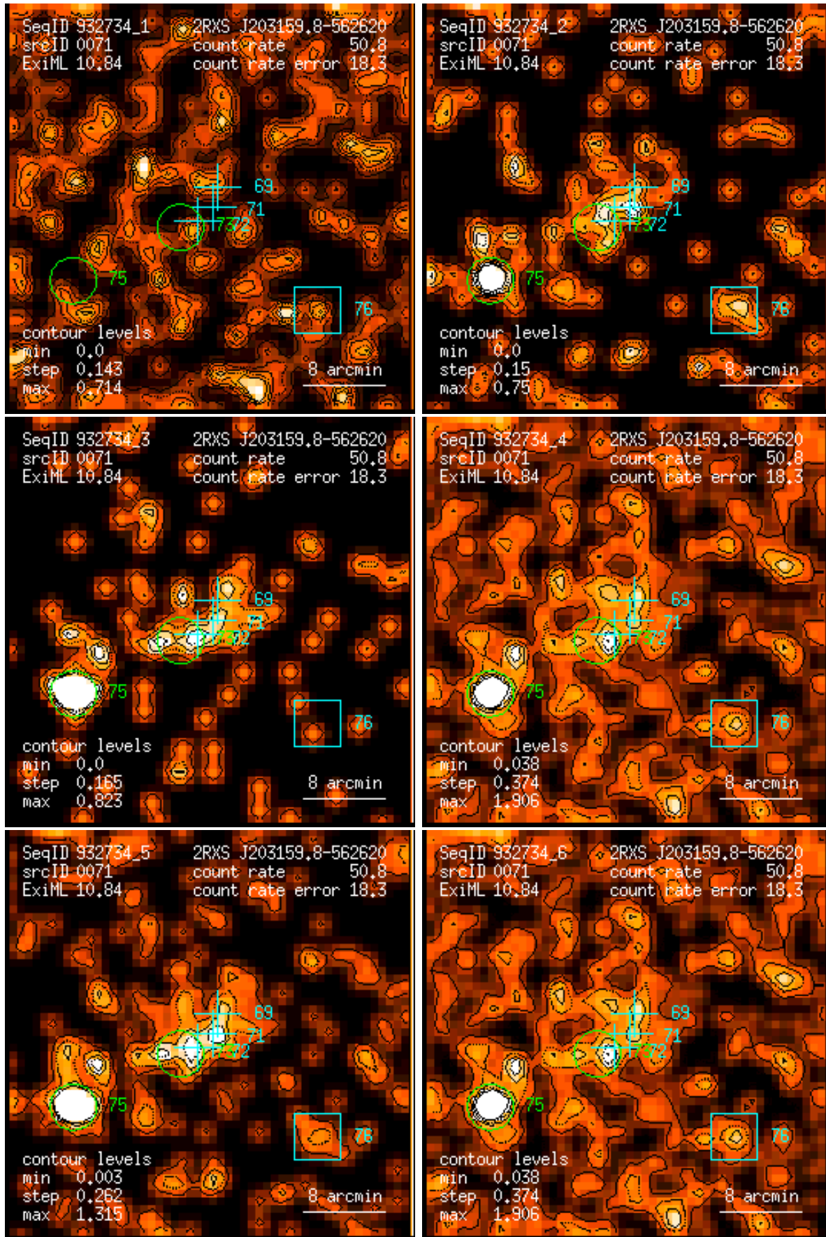
Figure 71: RASS 932734: detection 0071: band rate images, Gaussian filter: (1) PSPC channels 11 – 41, (2) 52 – 90, (3) 91 – 201, (4) 11 – 235, (5) 52 – 201, (6) 11 – 201. Broad band rates in counts/ks. Band rate contour levels in counts/ks/arcmin 2 .
