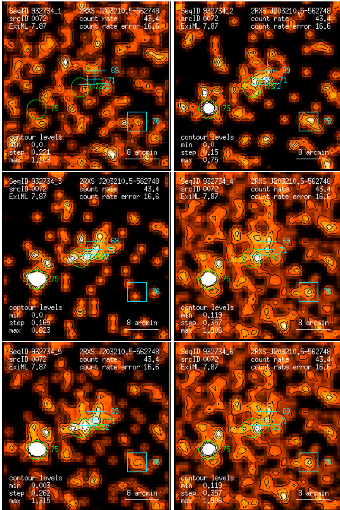
Figure 72: RASS 932734: detection 0072: band rate images, Gaussian filter: (1) PSPC channels 11 – 41, (2) 52 – 90, (3) 91 – 201, (4) 11 – 235, (5) 52 – 201, (6) 11 – 201. Broad band rates in counts/ks. Band rate contour levels in counts/ks/arcmin 2 .
