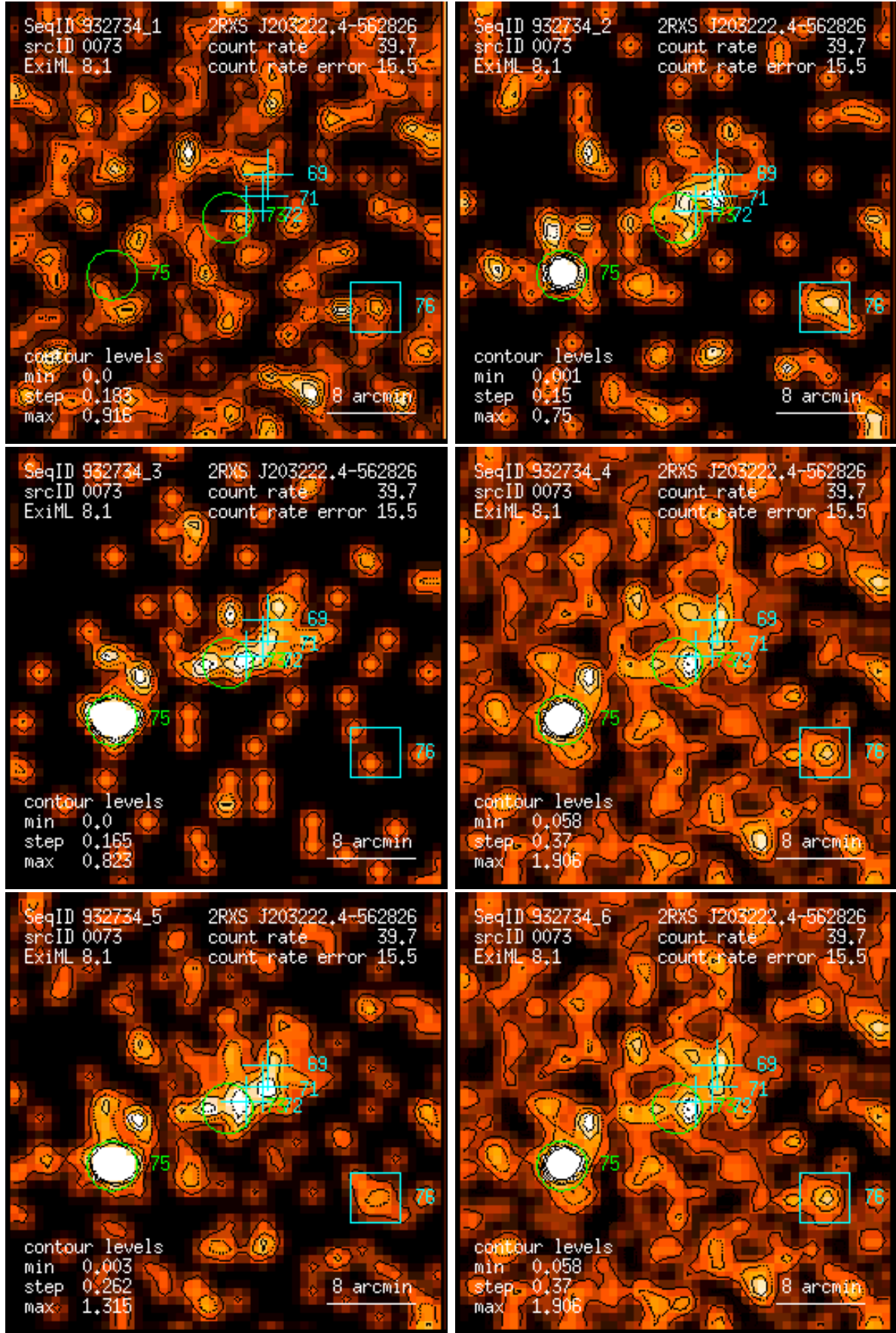
Figure 73: RASS 932734: detection 0073: band rate images, Gaussian filter: (1) PSPC channels 11 – 41, (2) 52 – 90, (3) 91 – 201, (4) 11 – 235, (5) 52 – 201, (6) 11 – 201. Broad band rates in counts/ks. Band rate contour levels in counts/ks/arcmin 2 .
