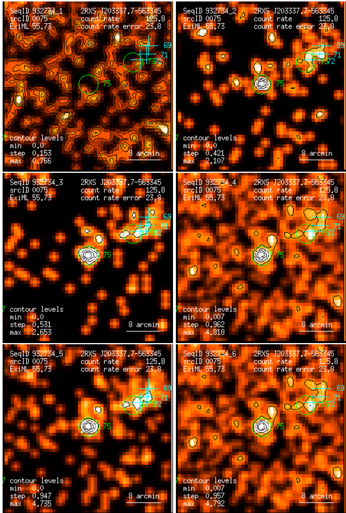
Figure 75: RASS 932734: detection 0075: band rate images, Gaussian filter: (1) PSPC channels 11 – 41, (2) 52 – 90, (3) 91 – 201, (4) 11 – 235, (5) 52 – 201, (6) 11 – 201. Broad band rates in counts/ks. Band rate contour levels in counts/ks/arcmin 2 .
