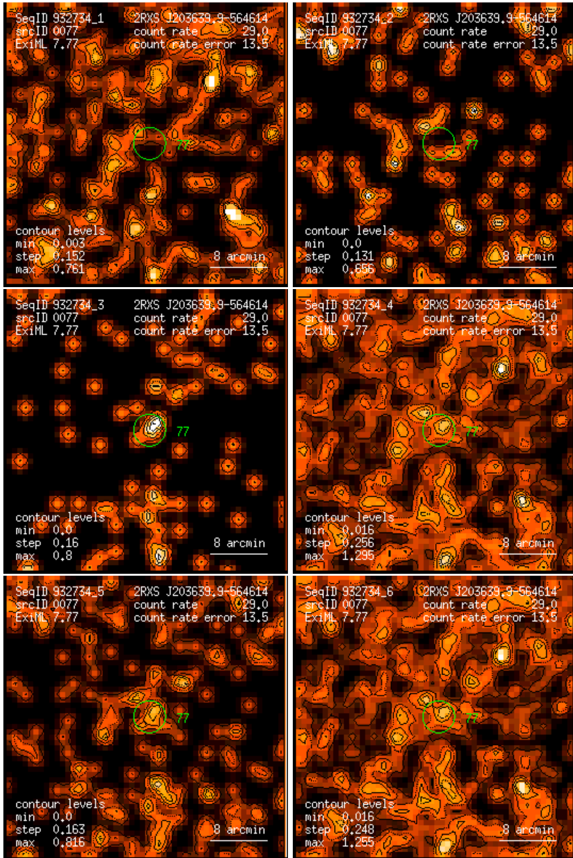
Figure 77: RASS 932734: detection 0077: band rate images, Gaussian filter: (1) PSPC channels 11 – 41, (2) 52 – 90, (3) 91 – 201, (4) 11 – 235, (5) 52 – 201, (6) 11 – 201. Broad band rates in counts/ks. Band rate contour levels in counts/ks/arcmin 2 .
