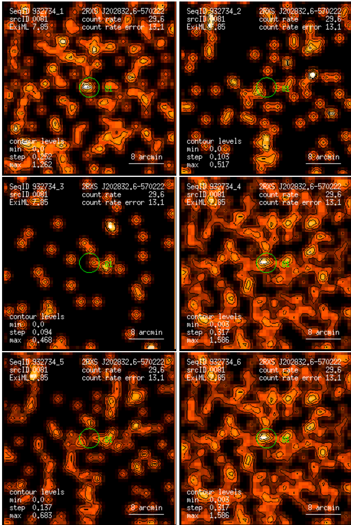
Figure 81: RASS 932734: detection 0081: band rate images, Gaussian filter: (1) PSPC channels 11 – 41, (2) 52 – 90, (3) 91 – 201, (4) 11 – 235, (5) 52 – 201, (6) 11 – 201. Broad band rates in counts/ks. Band rate contour levels in counts/ks/arcmin 2 .
