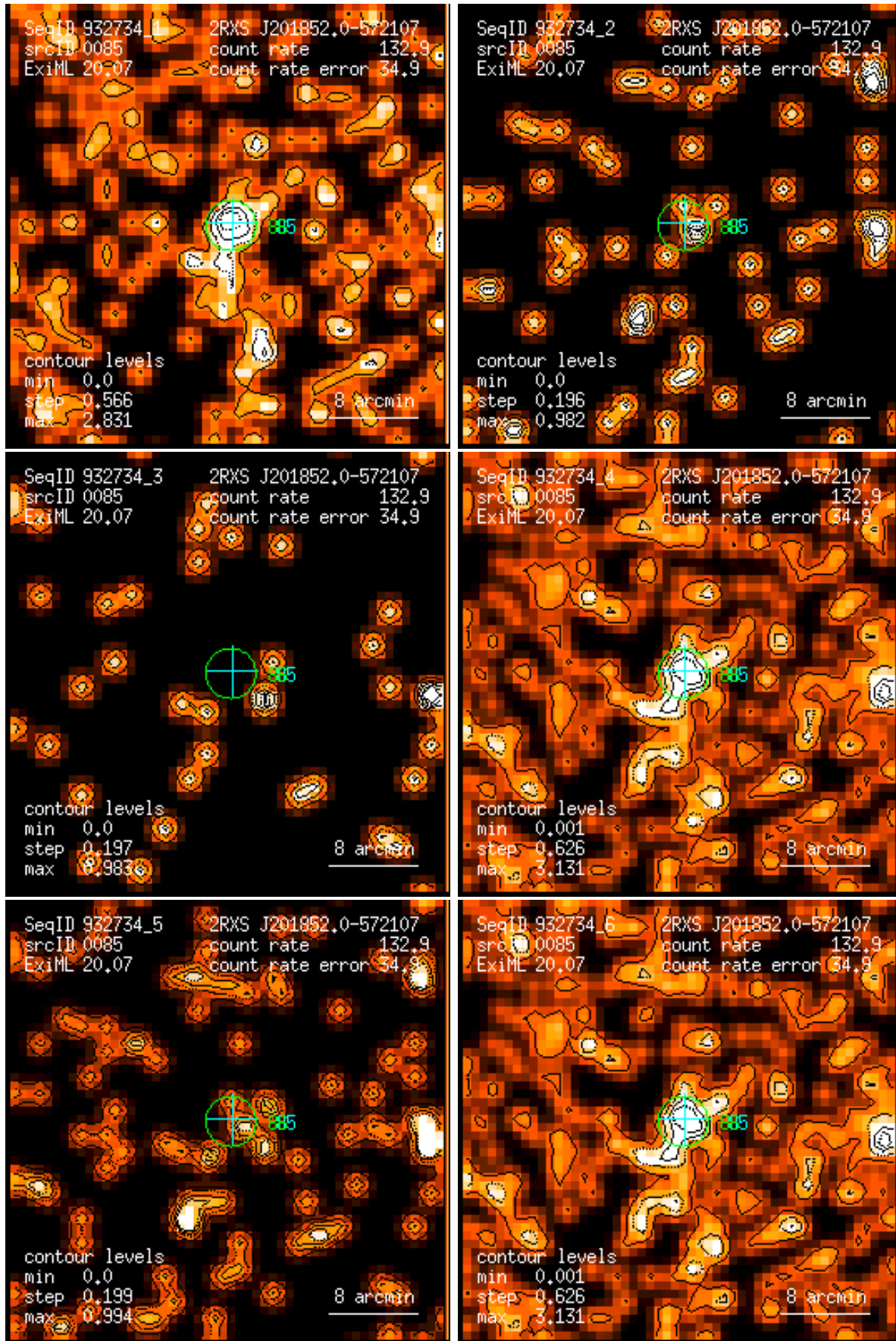
Figure 85: RASS 932734: detection 0085: band rate images, Gaussian filter: (1) PSPC channels 11 – 41, (2) 52 – 90, (3) 91 – 201, (4) 11 – 235, (5) 52 – 201, (6) 11 – 201. Broad band rates in counts/ks. Band rate contour levels in counts/ks/arcmin 2 .
