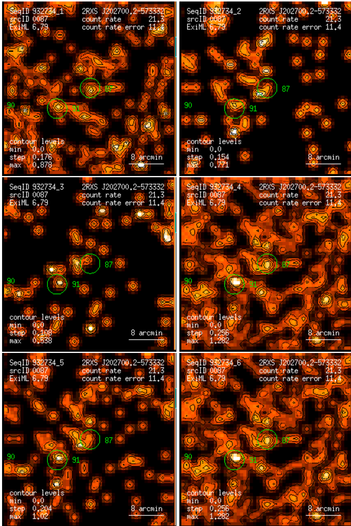
Figure 87: RASS 932734: detection 0087: band rate images, Gaussian filter: (1) PSPC channels 11 – 41, (2) 52 – 90, (3) 91 – 201, (4) 11 – 235, (5) 52 – 201, (6) 11 – 201. Broad band rates in counts/ks. Band rate contour levels in counts/ks/arcmin 2 .
