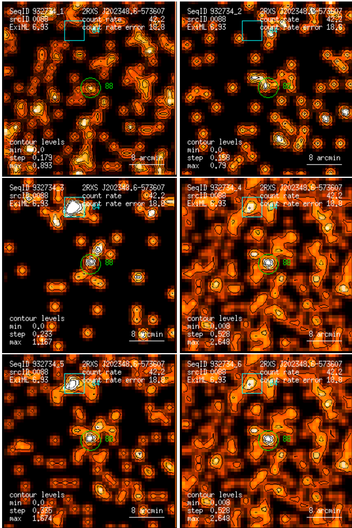
Figure 88: RASS 932734: detection 0088: band rate images, Gaussian filter: (1) PSPC channels 11 – 41, (2) 52 – 90, (3) 91 – 201, (4) 11 – 235, (5) 52 – 201, (6) 11 – 201. Broad band rates in counts/ks. Band rate contour levels in counts/ks/arcmin 2 .
