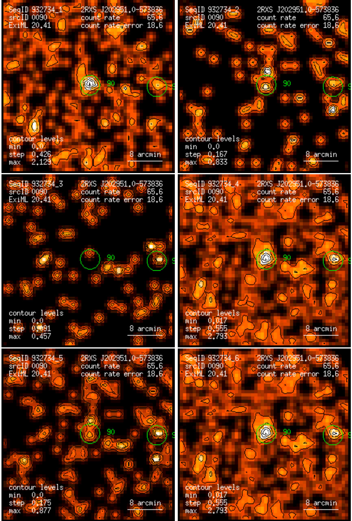
Figure 90: RASS 932734: detection 0090: band rate images, Gaussian filter: (1) PSPC channels 11 – 41, (2) 52 – 90, (3) 91 – 201, (4) 11 – 235, (5) 52 – 201, (6) 11 – 201. Broad band rates in counts/ks. Band rate contour levels in counts/ks/arcmin 2 .
