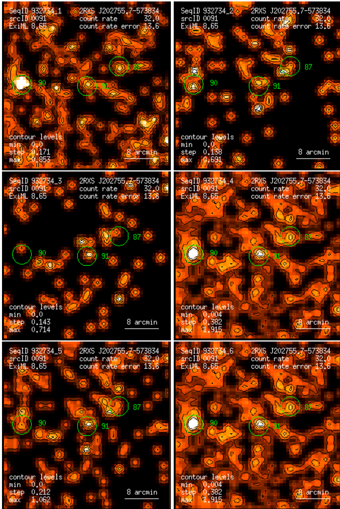
Figure 91: RASS 932734: detection 0091: band rate images, Gaussian filter: (1) PSPC channels 11 – 41, (2) 52 – 90, (3) 91 – 201, (4) 11 – 235, (5) 52 – 201, (6) 11 – 201. Broad band rates in counts/ks. Band rate contour levels in counts/ks/arcmin 2 .
