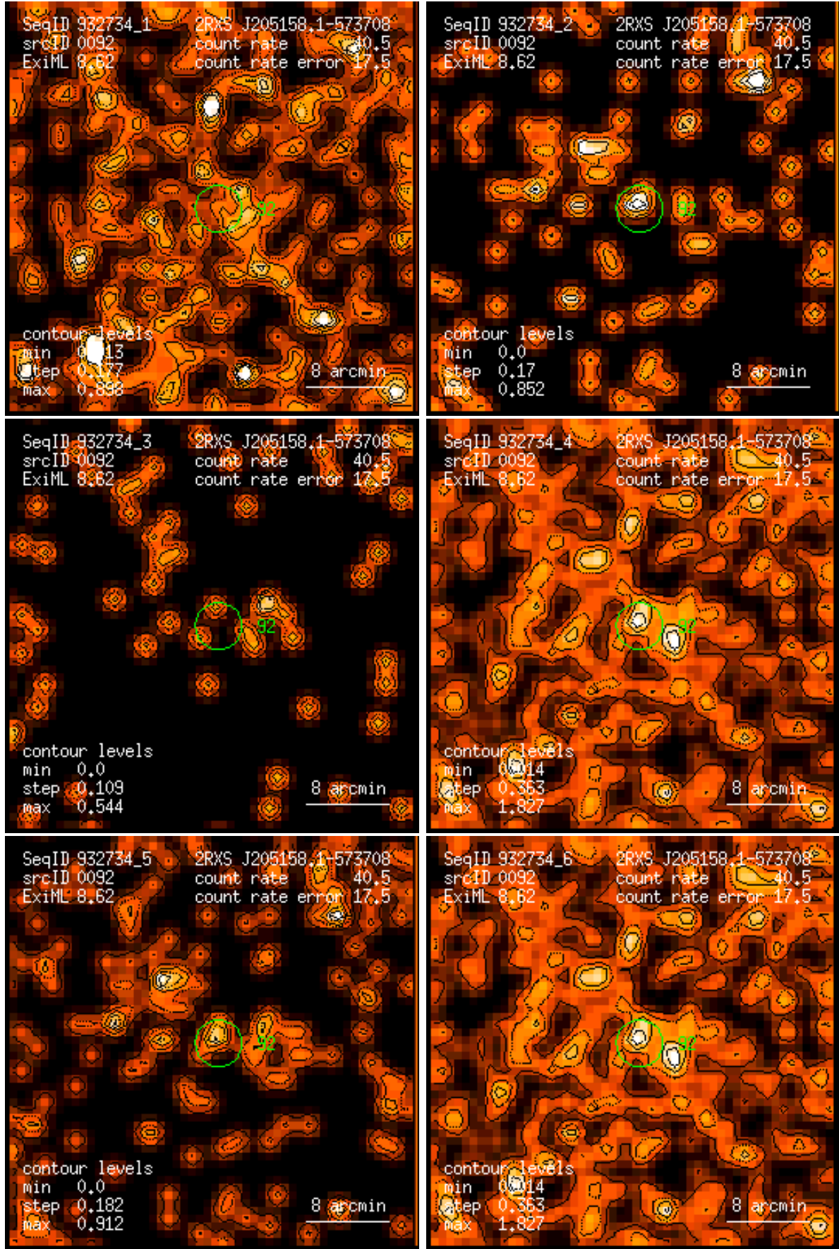
Figure 92: RASS 932734: detection 0092: band rate images, Gaussian filter: (1) PSPC channels 11 – 41, (2) 52 – 90, (3) 91 – 201, (4) 11 – 235, (5) 52 – 201, (6) 11 – 201. Broad band rates in counts/ks. Band rate contour levels in counts/ks/arcmin 2 .
