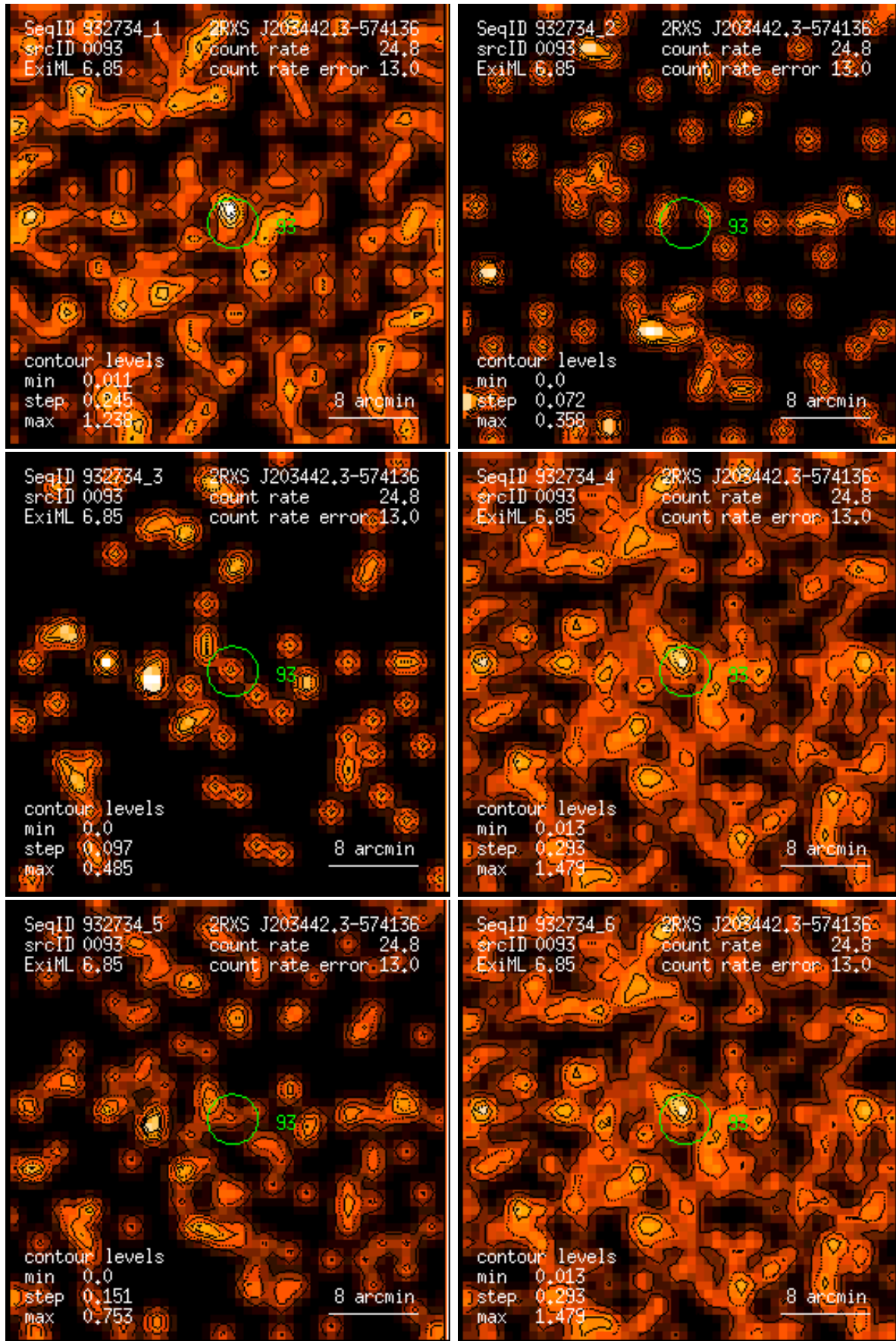
Figure 93: RASS 932734: detection 0093: band rate images, Gaussian filter: (1) PSPC channels 11 – 41, (2) 52 – 90, (3) 91 – 201, (4) 11 – 235, (5) 52 – 201, (6) 11 – 201. Broad band rates in counts/ks. Band rate contour levels in counts/ks/arcmin 2 .
