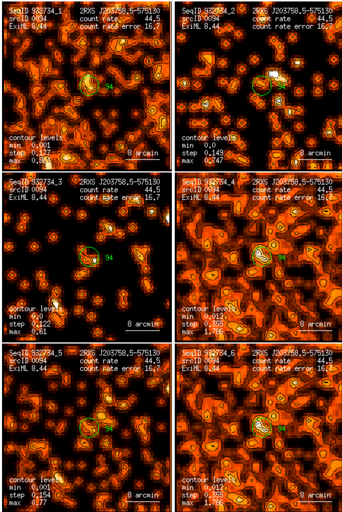
Figure 94: RASS 932734: detection 0094: band rate images, Gaussian filter: (1) PSPC channels 11 – 41, (2) 52 – 90, (3) 91 – 201, (4) 11 – 235, (5) 52 – 201, (6) 11 – 201. Broad band rates in counts/ks. Band rate contour levels in counts/ks/arcmin 2 .
