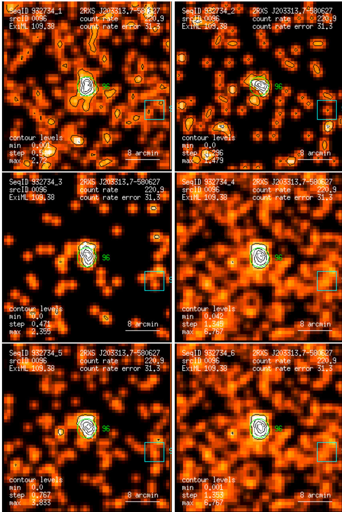
Figure 96: RASS 932734: detection 0096: band rate images, Gaussian filter: (1) PSPC channels 11 – 41, (2) 52 – 90, (3) 91 – 201, (4) 11 – 235, (5) 52 – 201, (6) 11 – 201. Broad band rates in counts/ks. Band rate contour levels in counts/ks/arcmin 2 .
