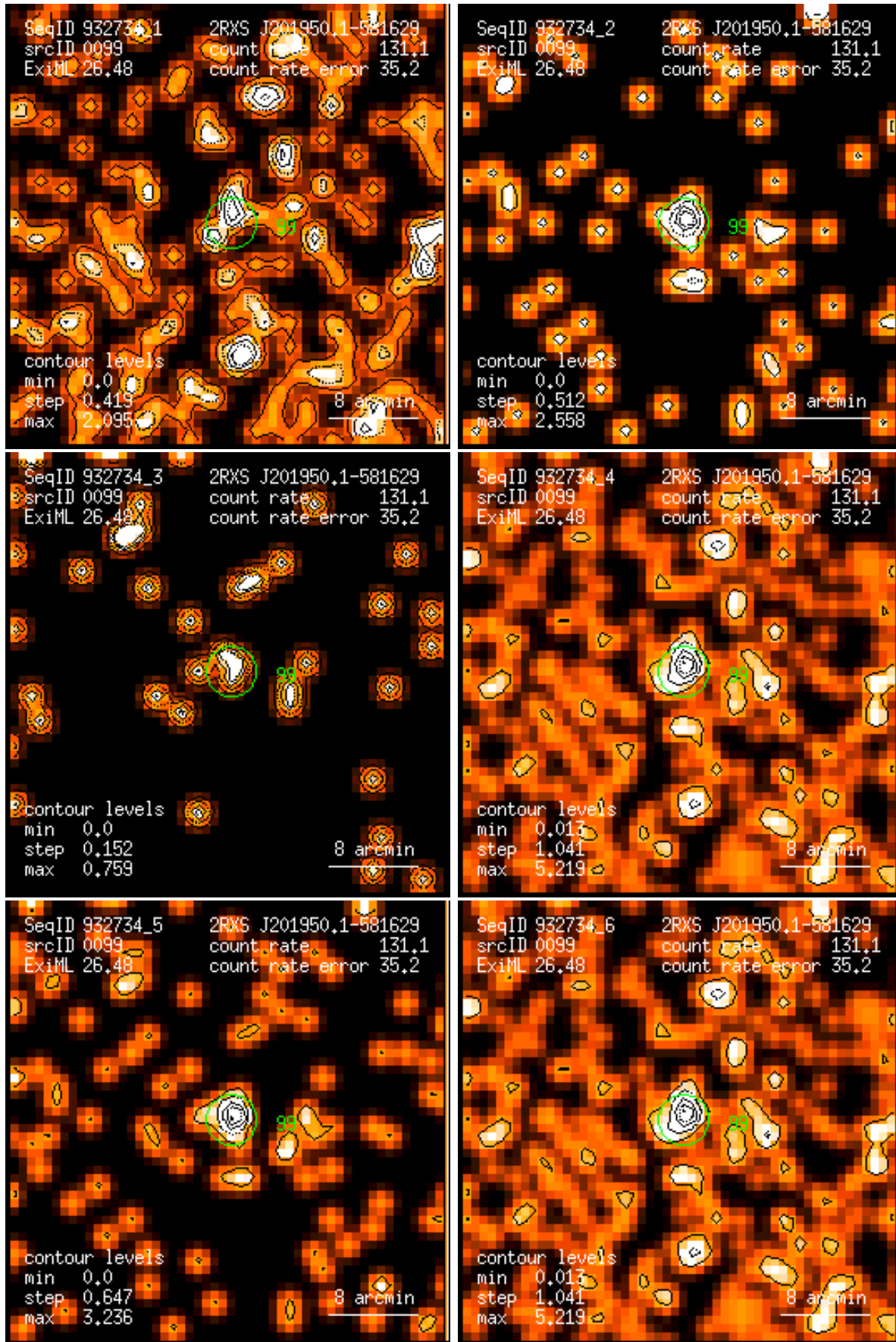
Figure 99: RASS 932734: detection 0099: band rate images, Gaussian filter: (1) PSPC channels 11 – 41, (2) 52 – 90, (3) 91 – 201, (4) 11 – 235, (5) 52 – 201, (6) 11 – 201. Broad band rates in counts/ks. Band rate contour levels in counts/ks/arcmin 2 .
