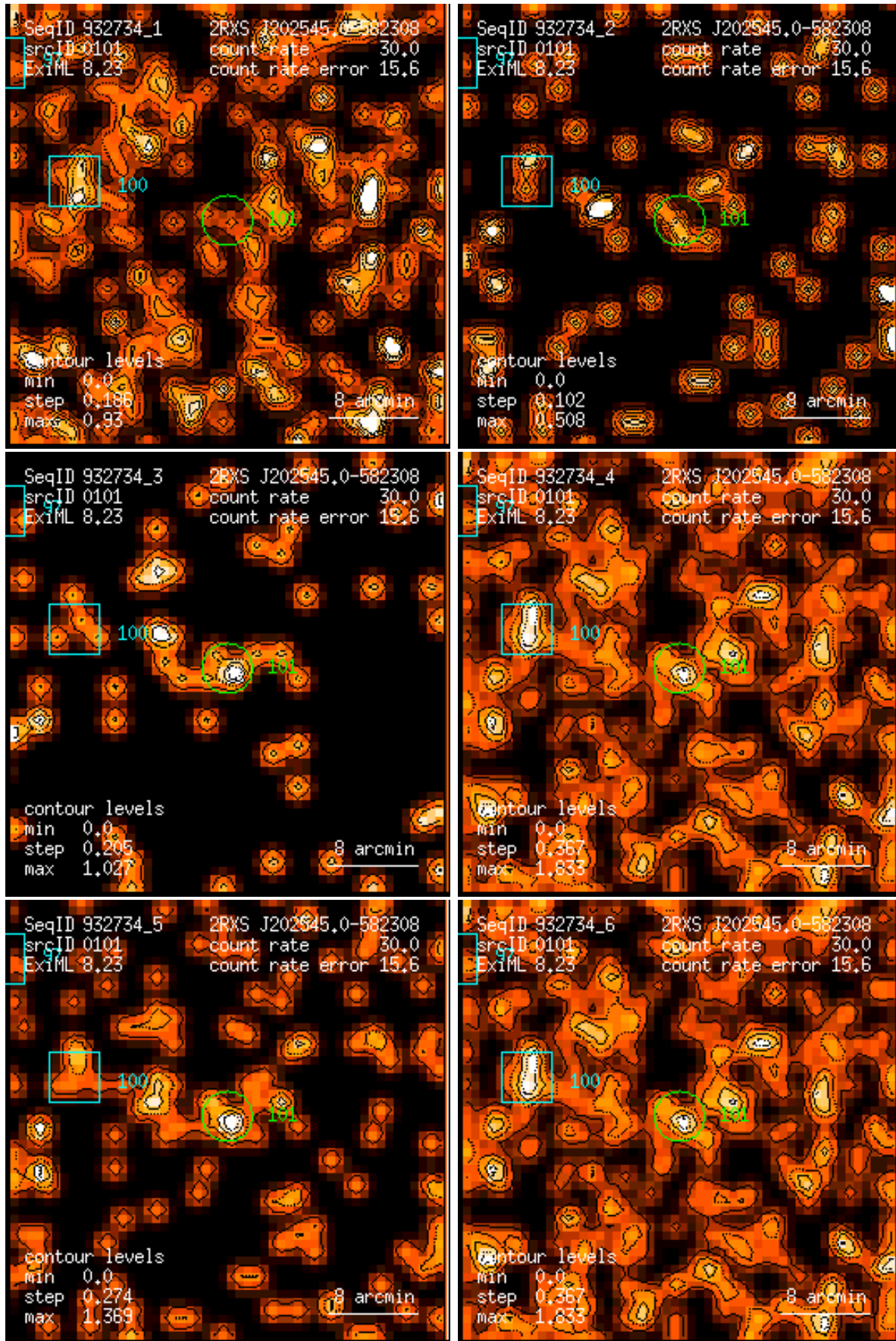
Figure 101: RASS 932734: detection 0101: band rate images, Gaussian filter: (1) PSPC channels 11 – 41, (2) 52 – 90, (3) 91 – 201, (4) 11 – 235, (5) 52 – 201, (6) 11 – 201. Broad band rates in counts/ks. Band rate contour levels in counts/ks/arcmin 2 .
