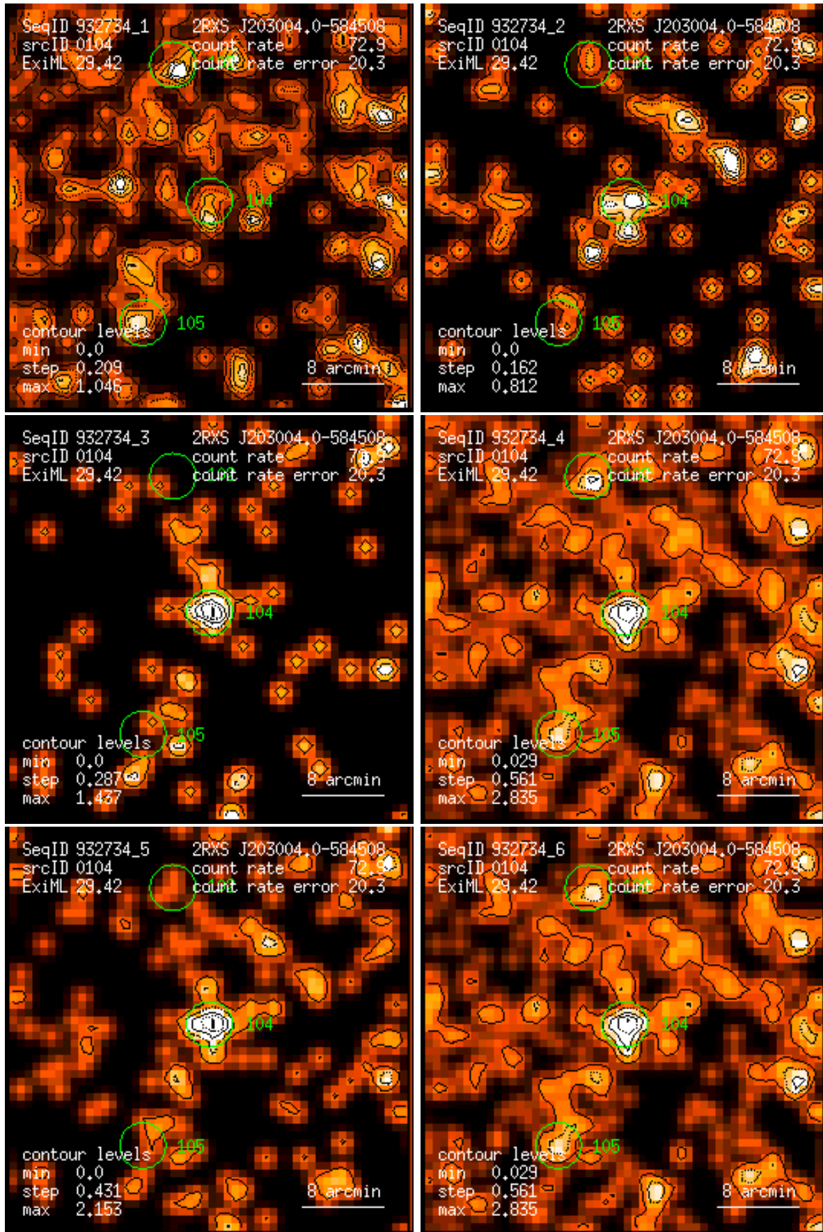
Figure 104: RASS 932734: detection 0104: band rate images, Gaussian filter: (1) PSPC channels 11 – 41, (2) 52 – 90, (3) 91 – 201, (4) 11 – 235, (5) 52 – 201, (6) 11 – 201. Broad band rates in counts/ks. Band rate contour levels in counts/ks/arcmin 2 .
