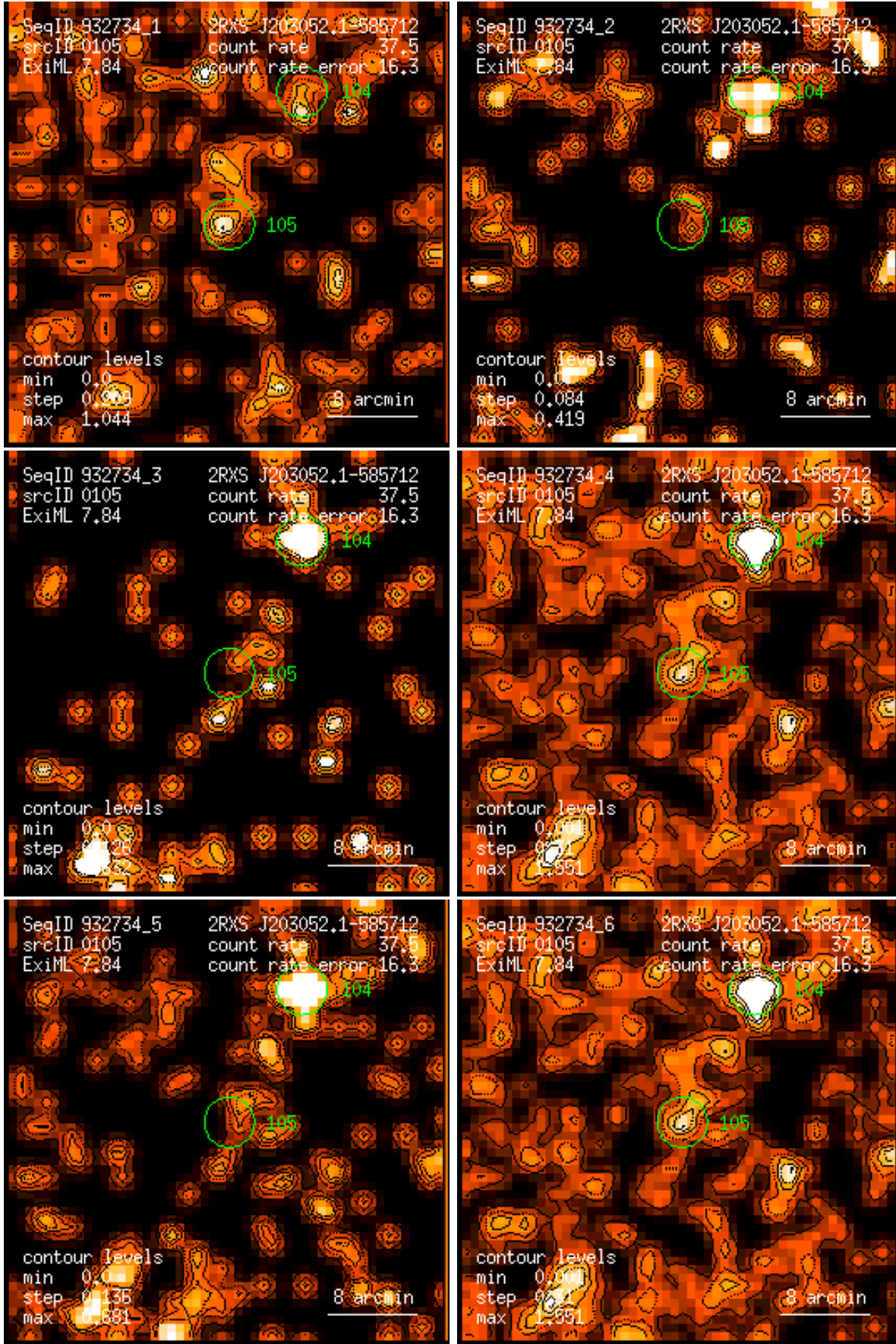
Figure 105: RASS 932734: detection 0105: band rate images, Gaussian filter: (1) PSPC channels 11 – 41, (2) 52 – 90, (3) 91 – 201, (4) 11 – 235, (5) 52 – 201, (6) 11 – 201. Broad band rates in counts/ks. Band rate contour levels in counts/ks/arcmin 2 .
