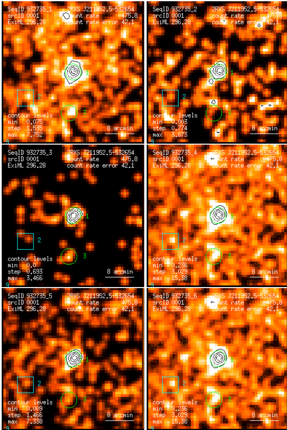
Figure 1: RASS 932735: detection 0001: band rate images, Gaussian filter: (1) PSPC channels 11 – 41, (2) 52 – 90, (3) 91 – 201, (4) 11 – 235, (5) 52 – 201, (6) 11 – 201. Broad band rates in counts/ks. Band rate contour levels in counts/ks/arcmin 2 .
