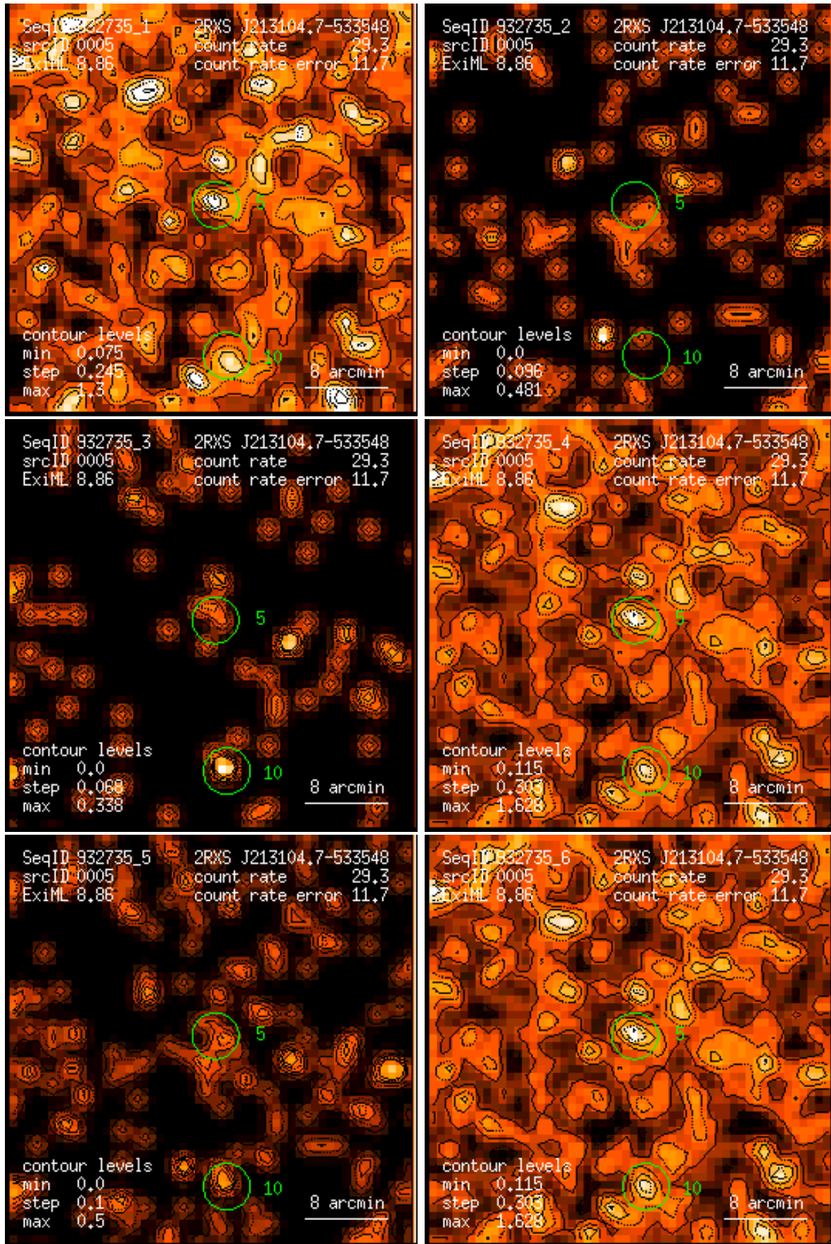
Figure 5: RASS 932735: detection 0005: band rate images, Gaussian filter: (1) PSPC channels 11 – 41, (2) 52 – 90, (3) 91 – 201, (4) 11 – 235, (5) 52 – 201, (6) 11 – 201. Broad band rates in counts/ks. Band rate contour levels in counts/ks/arcmin 2 .
