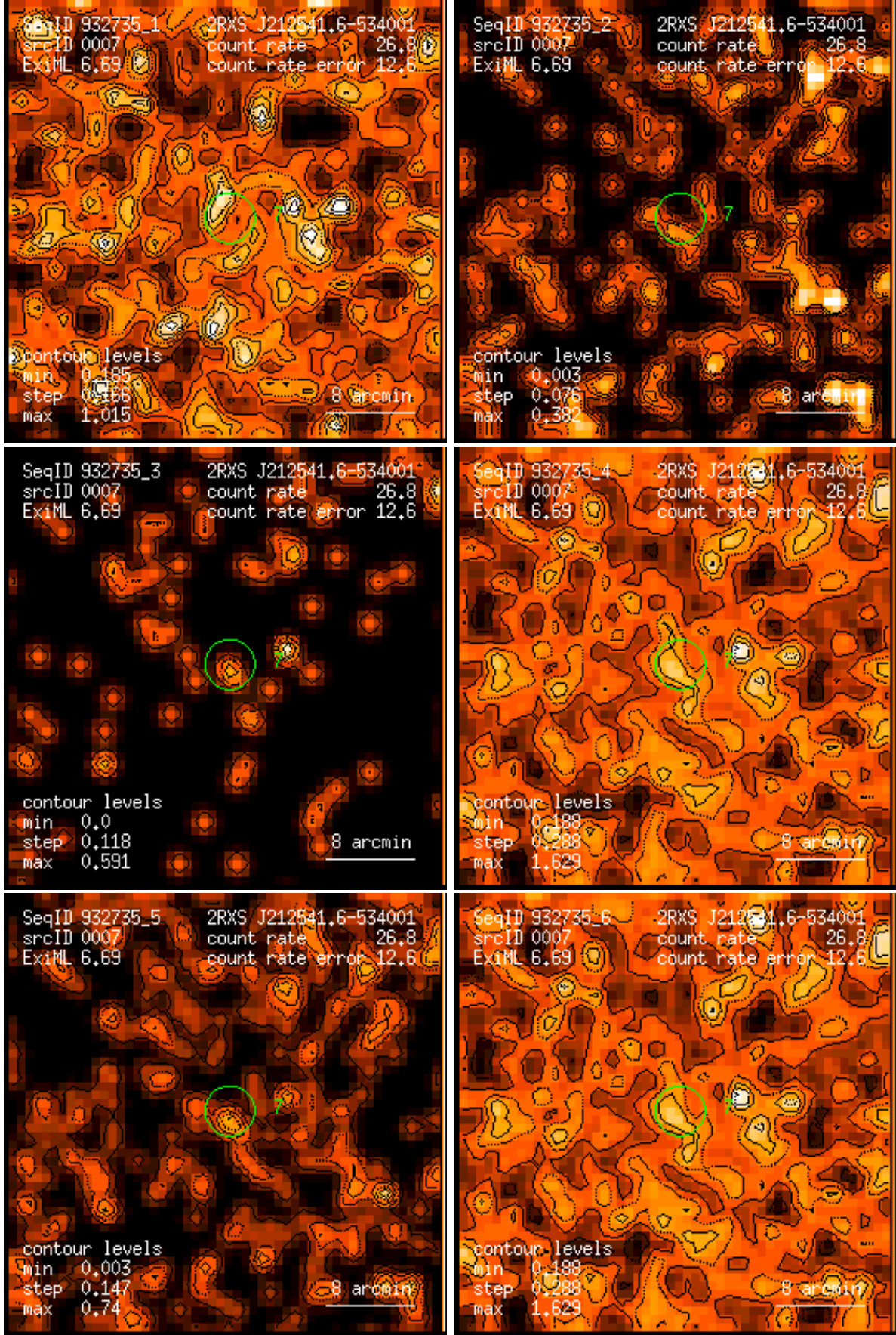
Figure 7: RASS 932735: detection 0007: band rate images, Gaussian filter: (1) PSPC channels 11 – 41, (2) 52 – 90, (3) 91 – 201, (4) 11 – 235, (5) 52 – 201, (6) 11 – 201. Broad band rates in counts/ks. Band rate contour levels in counts/ks/arcmin 2 .
